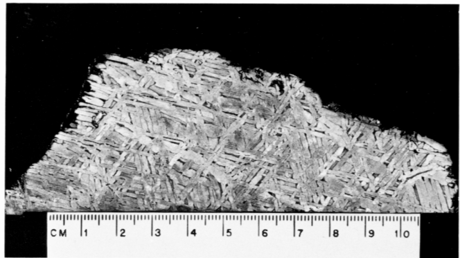
Figure 429. Campbellville (Tempe no. 351.1). This medium octahedrite is corroded and shows local exfoliation along Widmanstätten lamellae. Deep-etched. Scale bar in cm. (Courtesy C.B. Moore.)
