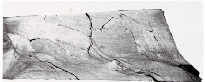
Figure 436. Campo del Cielo (U.S.N.M. no. 2253). Section through a mass that was heavily coldworked when the meteorite split in the atmosphere. Wavy sliplines and deformation bands cross the entire specimen. Etched. Scale bar 3 mm. S.I. neg. 1358G.
