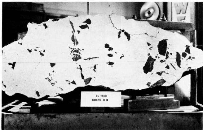
Figure 433. Campo del Cielo. The El Taco mass being cut in Mainz. Numerous large angular silicate-troilite-graphite aggregates. Length of slice 110 cm. (Courtesy Professor Hintenberger.) See also Figure 78.
