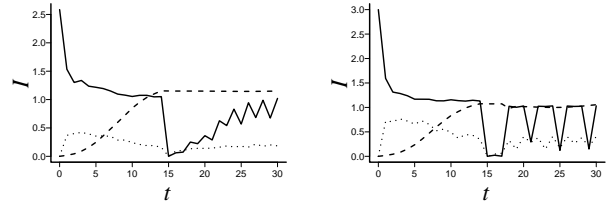
Figure 7: Information flows constructed by the best evolved 6-state (left) and 8-state (right) controller pairs. Solid line – I(M_0; M_t) , dashed – I(M_0; B_t) , dotted – I(R_0; M_t) .
