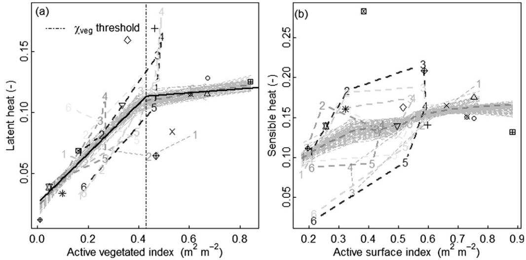
FIG. 8. Mean midday ratios of (a) Q_F/Q\downarrow and (b) Q_H/Q\downarrow as a function of the mean midday \chi_{veg} and \chi_{tot} values, respectively. The nonlinear regression (thick black line) for (a) is found in Eq. (27). For key, see Fig. 7.
