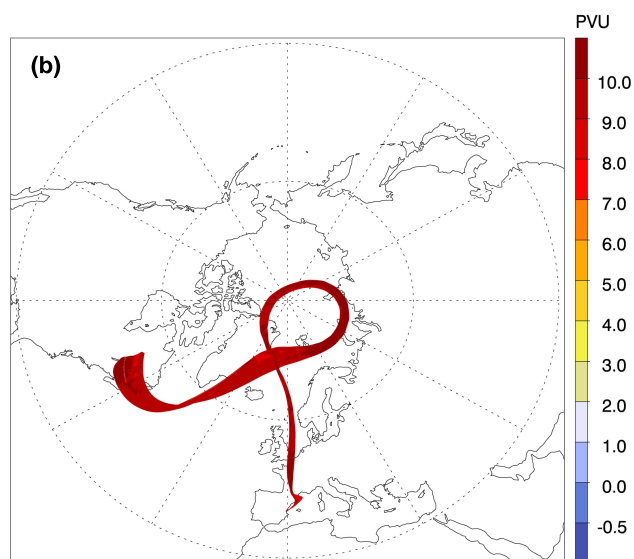
Fig. 7. 10-day backward trajectories along the flight path arriving between 09:00 UTC and 09:24 UTC at the flight path in flight segment I (a) and between 10:24 and 10:48 UTC in flight segment II (b). The color code indicates the PV of the air.
