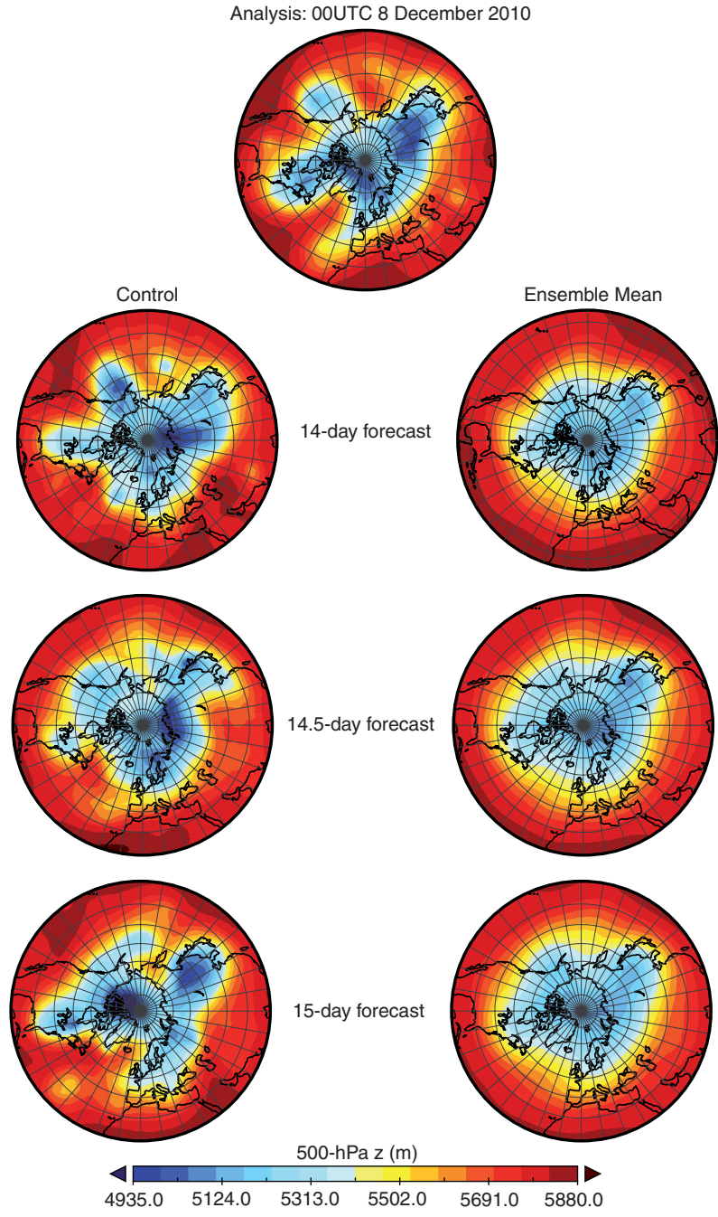
Fig. 6. The same as Fig. 5 but for the 14-, 14.5- and 15-d forecasts.
