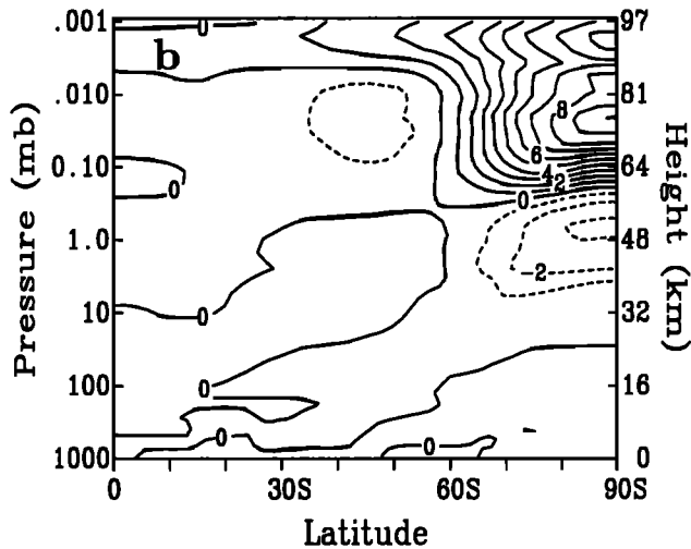
Figure 7. Zonally averaged fields appearing in (20), (a) (\Delta T_f - \Delta T_i)/\tau , contour interval of 0.1 \text{ K d}^{-1} , and (b) (\Delta Q_{ir}) , contour interval of 1 \text{ K d}^{-1} . Differences between the CMAM control run and the wave drag run are denoted by \Delta .
