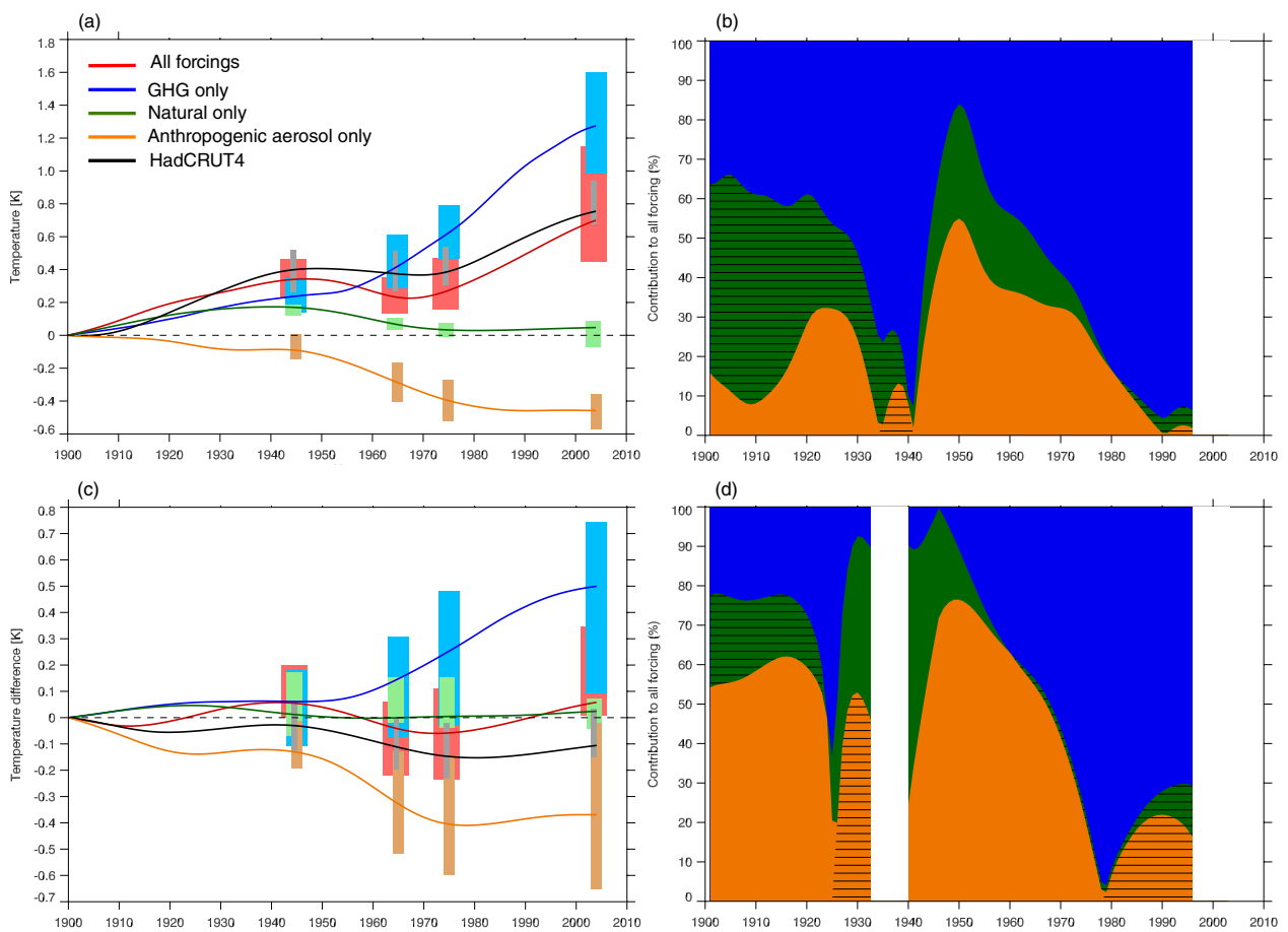
Figure 3. Non-linear trends (where the trend is the sum of the last IMF and the residual) from single forcing runs and observations for (a) global-mean annual-mean near-surface temperature; (c) annual-mean inter-hemispheric temperature difference. For model data, solid lines show the ensemble mean for each run, shading shows the absolute range of the instantaneous values from individual ensemble members (shown in bold in table 1) at the designated time. For HadCRUT4, the solid line shows the median of 100 ensemble members, and shading shows uncertainty resulting from measurement and sampling error, and coverage uncertainty (see Morice et al (2012) for further details of the uncertainty). Contributions from anthropogenic aerosol (sulfate, black carbon, and organic carbon), natural (solar and volcanic), and greenhouse gas forcing to the rate of change in (b) global-mean annual-mean near-surface temperature; (d) annual-mean inter-hemispheric temperature difference. No data is shown when the linear sum of the single forcing response is a poor approximation of the all forcing experiment.
