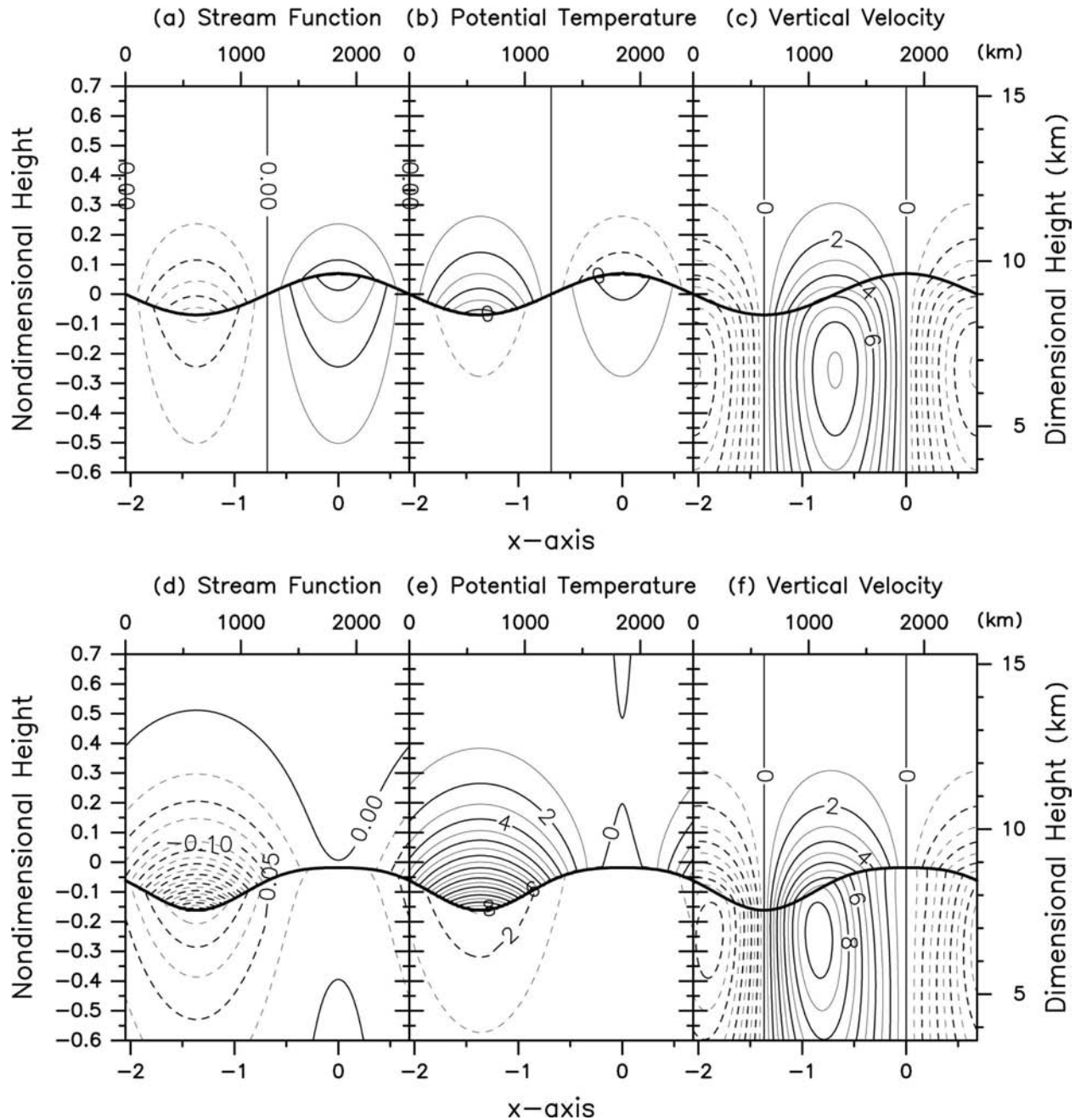
FIG. 12. Zonal cross sections of (a), (d) nondimensional streamfunction, (b), (e) dimensional potential temperature, and (c), (f) vertical velocity of (a)–(c) QG and (d)–(f) QG +1 solutions. Contour intervals are 0.025 in (a) and (d), 1 K in (b) and (e), and 1 mm s -1 in (c) and (f). Dashed contours represent negative values. Thick solid lines represent the tropopause. Top axis represents a horizontal distance.
