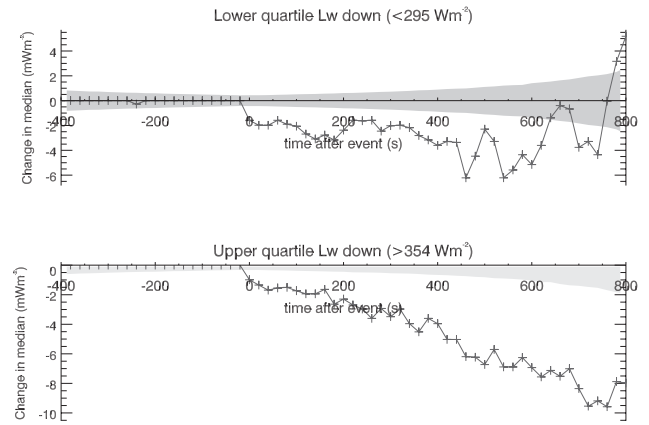
Figure 4. Change in median filter radiometer output (similar to the top panel of figure 3), sorted by downwelling longwave radiation. The upper panel shows the lower quartile ( <295 \text{ Wm}^{-2} ), 6295 events, and the lower panel the upper quartile ( >354 \text{ Wm}^{-2} ), 8164 events. The shaded region indicates the natural variability expected for the number of points in the composite, determined from periods during which no high-energy particle events were recorded (as for figure 3).
