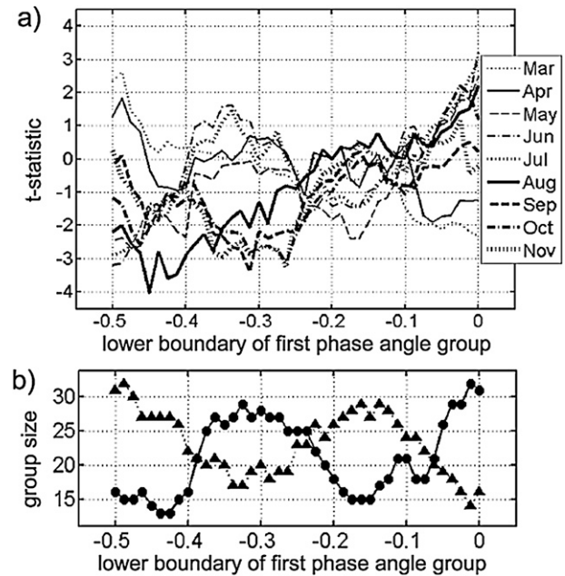
FIG. 13. As in Fig. 12, but for CMAM.
