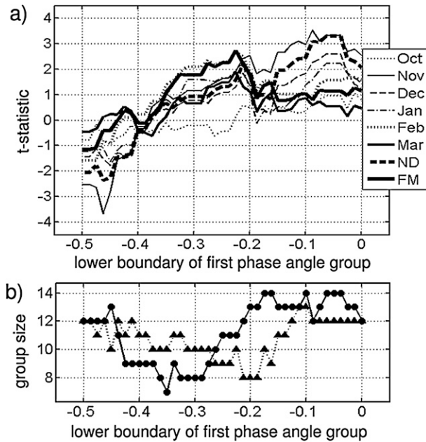
FIG. 8. (a) The t statistic for ERA-40 monthly or bimonthly \Delta\bar{u} at 60°N, 50 hPa (21 km) for varying \psi^G - \tilde{\psi}^G pairs; ND and FM denote November–December and February–March averages, respectively. The horizontal axis is labeled using the lower boundary value of the \psi^G group. (b) Sizes of the opposing groups for each \psi^G - \tilde{\psi}^G pair shown in (a); circles (triangles) indicate the size of the \psi^G ( \tilde{\psi}^G ) group.
