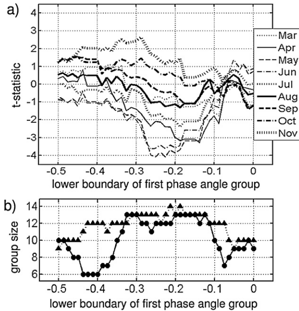
FIG. 12. As in Fig. 8, but for the SH. (a) The t statistic for ERA-40 \Delta\bar{u} at 30 hPa (25 km), averaged over 50^{\circ} – 60^{\circ} S [weighted by \cos(\phi) ], for varying \psi^G - \tilde{\psi}^G pairs.
