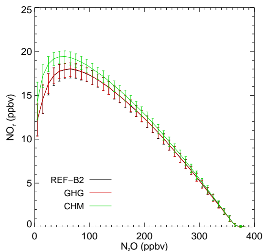
Fig. 7. The relationship between instantaneous concentrations of N 2 O and reactive nitrogen (NO y ) between approximately 150 and 1.0 hPa and 15° S to 15° N for the years 2080 and 2083. Data is taken from one member from each of the three experiments, sampled three times a month, and has been binned according to N 2 O concentration. Each data point shows the mean concentration of NO y in each bin, with the vertical bars giving the 10th and 90th percentiles.
