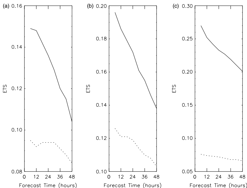
Figure 10. Equitable Threat Score (ETS) as a function of forecast time, for the operational North Atlantic and European Model (NAE; solid line) and for the global model (dotted line), averaged over the period December 2006 – February 2007. All stations in the NAE model domain were used. Curves show data for thresholds of (a) 200 m, (b) 1000 m and (c) 5000 m. For interpretation, see section 4.3.
