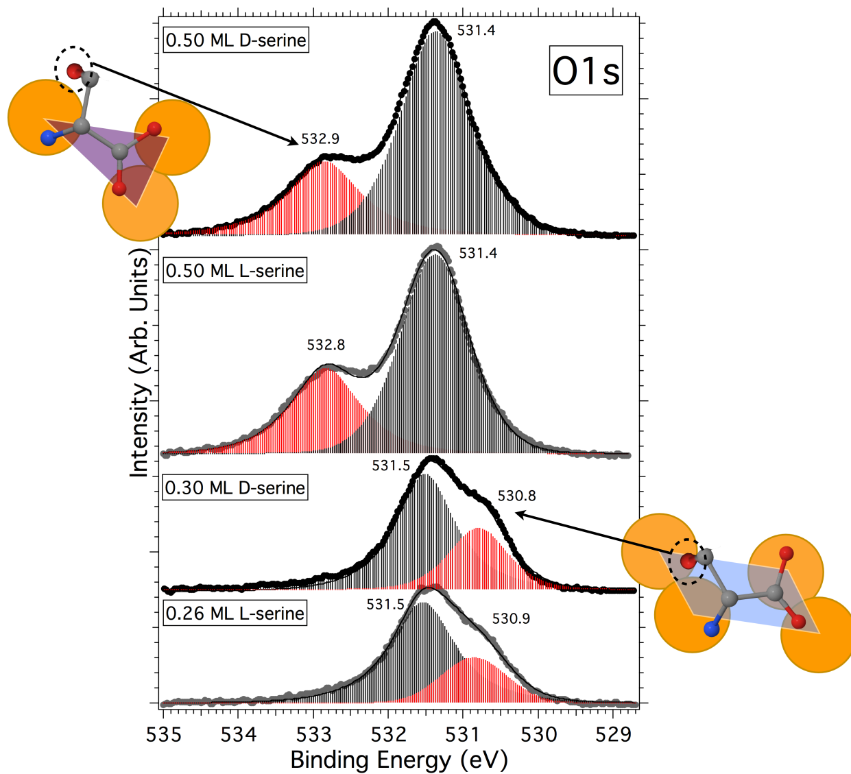
Figure 3: O 1s XP spectra of different coverages of L and D-serine adsorbed on \text{Cu}\{531\}^S (photon energy=630 eV). The insets indicate the likely adsorption-bond coordination. For clarity, hydrogen atoms are omitted in the diagrams.
