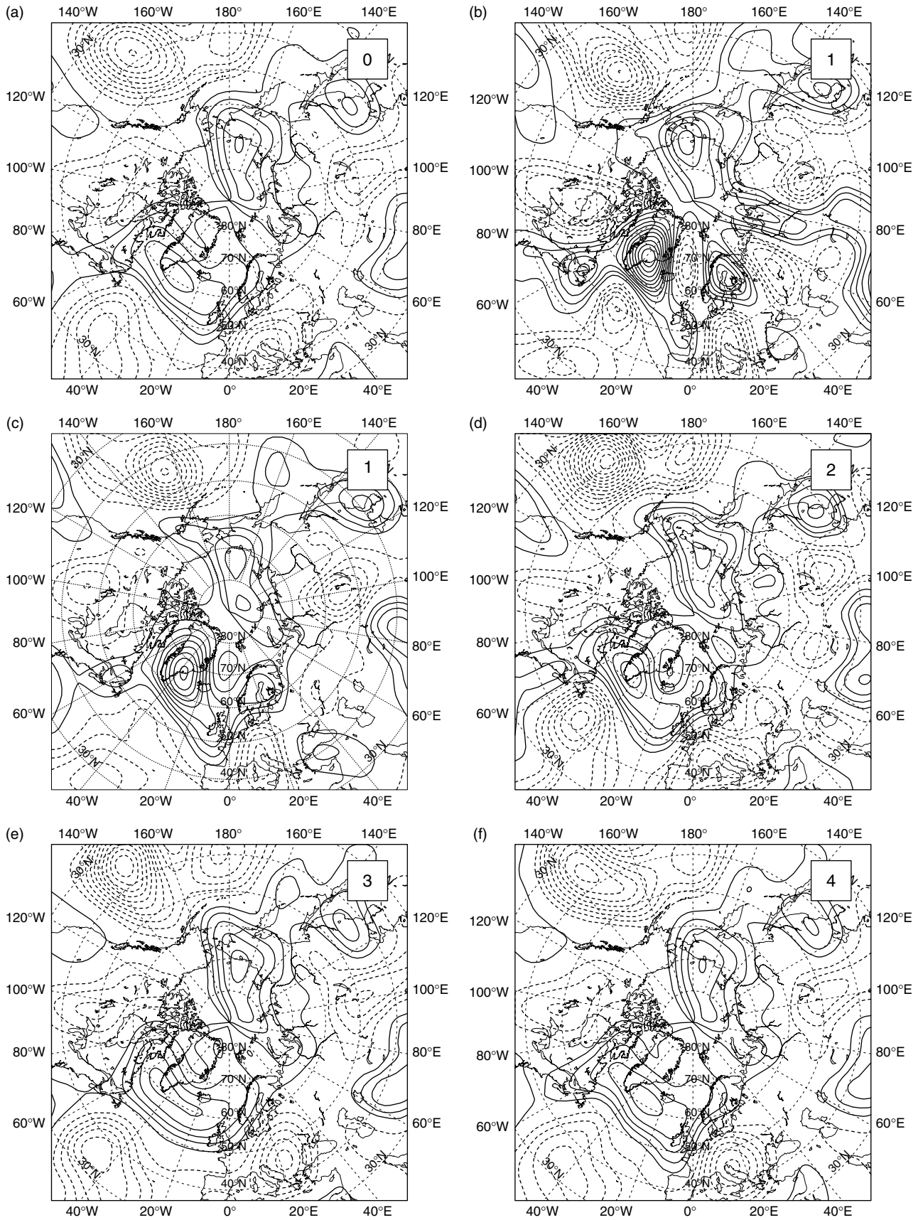
Figure 1. Streamfunction perturbation at 500 hPa after 2 days using (a) the nonlinear model \mathbf{x} , (b) the standard tangent linear model with \dot{\mathbf{x}}^0(t) = 0 , and the iterative relinearization method with \dot{\mathbf{x}}^0(t) = \mathbf{x}_0 for iterations (c) 1, (d) 2, (e) 3 and (f) 4. The initial condition for the perturbed run and the control run are 100 days apart. The contour interval is 1 \times 10^{-3} \Omega a^2 in all panels (with a and \Omega the average radius and the angular velocity of the Earth, respectively), with positive values solid and negative values dashed.
