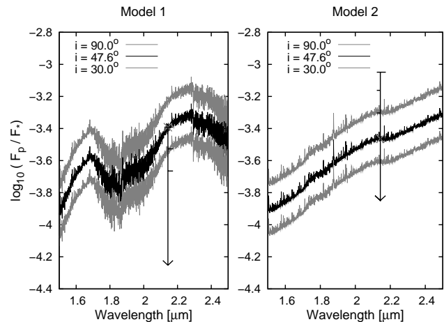
Figure 4. Model and 2.14 \mu\text{m} planet/Star flux ratios for HD 179949b. Shown are models for model 1, absorption (left) and model 2, TiO/VO stratosphere, emission spectrum (right). Some apparent emission features are due to stellar absorption lines and result from dividing the planet spectrum by the stellar spectrum. The black crosses indicate the mean model flux over the wavelength of observations for the most probable inclination. Upper limits corresponding to the levels in Fig. 3 (99.9, 99 and 95.4 per cent) are marked by horizontal bars (from top to bottom) for our analysis using each model. The 99.9 per cent observational upper limit is coincident with the mean flux level for the model 1 model. The width of the top horizontal bar in each case (99.9 per cent confidence) represents the wavelength range of the CRRES spectroscopic observations. For model 1, we can marginally exclude the model with 99.9 per cent confidence at the most probable inclination of 47.6°. For model 2 we are unable to exclude the model since the 95.4 per cent confidence level ( 2\text{-}\sigma ) is above the model flux ratio and artifacts are present between 2\text{-}\sigma and 1\text{-}\sigma (68.3 per cent confidence marked by the arrow).
