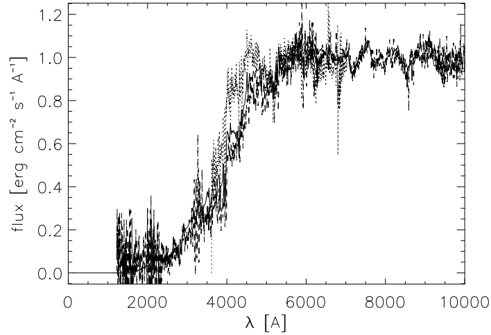
Figure 2. Comparison of Sb templates NGC3147 (dotted), NGC210 (dashed) with galaxy model t_* = 1 Gyr (solid). Fluxes are normalized at 5500 \text{ \AA} .
