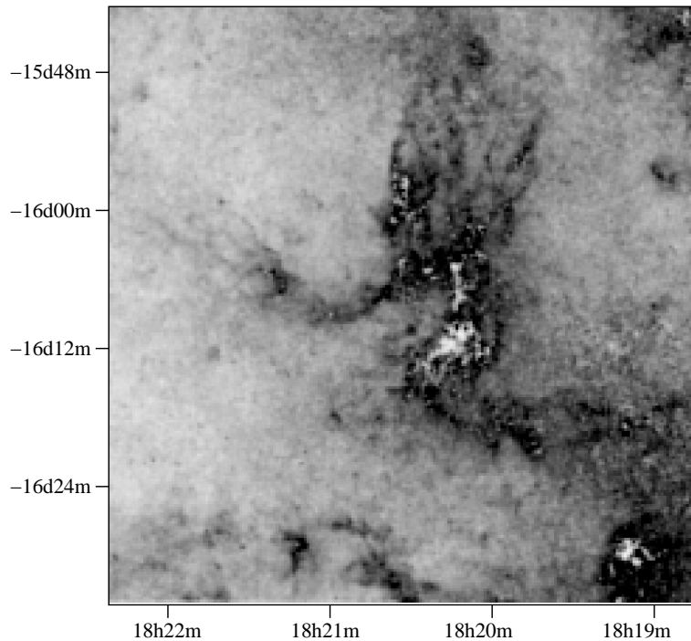
Figure 18. Extinction map of the M17 field, illustrating the “Omega” shape of the nebula. The greyscale runs from A_V=0 (white) to A_V=26 (black). The extinction for each star was derived from the (H-K) colour and the results were averaged in 15 arcsecond bins (see text). The white regions surrounded by black are places with very high extinction where only foreground stars are detected.
