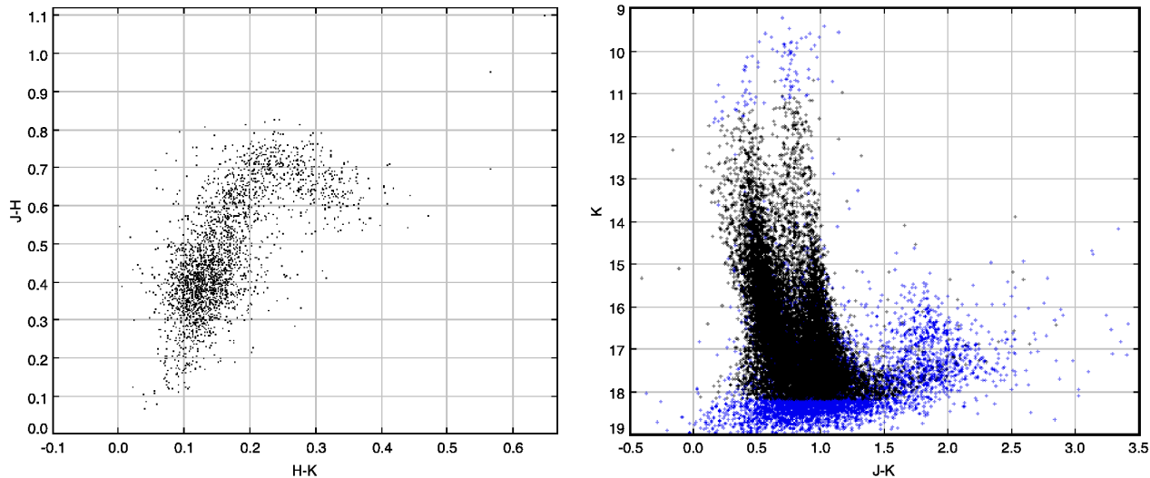
Figure 12. (l, b)=(171.1, 4.75) . This field lies on a line of sight almost directly opposite the Galactic centre and 4.75^\circ off the plane. The stellar populations are very different from those in figures 2 to 10: the right hand sequence of stars in the colour magnitude diagram is now dominated by nearby late K and M dwarfs, as opposed to red clump giants. Giants are more numerous than late K and M dwarfs only at m_K \lesssim 13 , but they are not clearly distinguished from the dwarfs in the colour magnitude diagram. The left hand sequence is dominated by F and G dwarfs. There are relatively few nearby bright early K dwarfs to bridge the gaps between the sequences (see figure 14). The two sequences join at faint magnitudes, where there is a substantial population of relatively distant early K, late K and early M dwarfs. The two colour diagram shows that there is little reddening in this field. The points plotted are selected in the same way as in figure 2.
