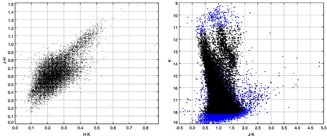
Figure 10. (l, b)=(98.4, 1) . The diagrams for this field appear very similar to those for (l, b)=(98.4, 0) , in term of reddening. This is consistent with expectations due to the presence of the northern warp, which creates an overdensity of stars and interstellar extinction above the plane at large Galactocentric distances, relative to what would be expected if the outer Galaxy were centred in the plane. The points plotted are selected in the same way as in figure 2.
