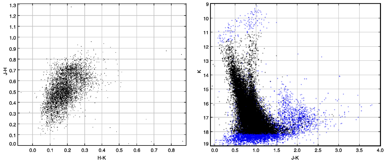
Figure 12. (l, b)=(171.1, 4.75) . This field lies on a line of sight almost directly opposite the Galactic centre and 4.75^\circ off the plane. The stellar populations are very different from those in figures 2 to 10: the right hand sequence of stars in the colour magnitude diagram is now dominated by nearby late K and M dwarfs, as opposed to red clump giants. Giants are more numerous than late K and M dwarfs only at m_K \lesssim 13 , but they are not clearly distinguished from the dwarfs in the colour magnitude diagram. The left hand sequence is dominated by F and G dwarfs. There are relatively few nearby bright early K dwarfs to bridge the gaps between the sequences (see figure 14). The two sequences join at faint magnitudes, where there is a substantial population of relatively distant early K, late K and early M dwarfs. The two colour diagram shows that there is little reddening in this field. The points plotted are selected in the same way as in figure 2.
