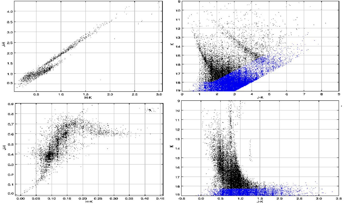
Figure 14. Besançon model results with synthetic errors. Upper panels: (l, b)=(31,0) . Lower panels (l, b)=(171.1, 4.75) . These models reproduce the data fairly well, although our use of synthetic errors based on the archival values has underestimated the true errors at bright magnitudes (see Appendix A2), causing the various stellar sequences to appear narrower than in the real data. The small, well defined sequence of rather red white dwarfs with m_K \sim 14 in the plots for (l, b)=(171.1, 4.75) is not observed in figure 13 (see text). The A type stars near the origin in the lower left panel are not measured by the GPS because they are saturated. Points with synthetic errors > 0.2 mag are plotted in blue.
