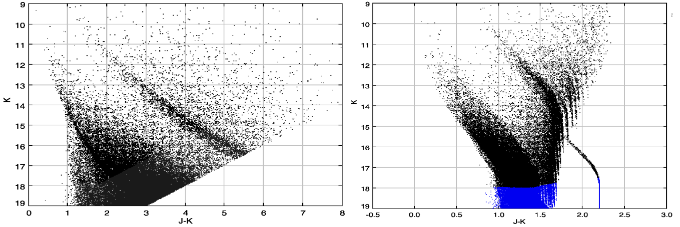
Figure 15. Besançon model K vs. (J-K) diagrams with no errors. Left panel: (l, b)=(31,0) . Right panel: (l, b)=(15,1) , showing the numerous sub-sequences of giant stars which comprise the red giant clump giant. The single diagonal sequence of white dwarfs at the lower right is not observed.
