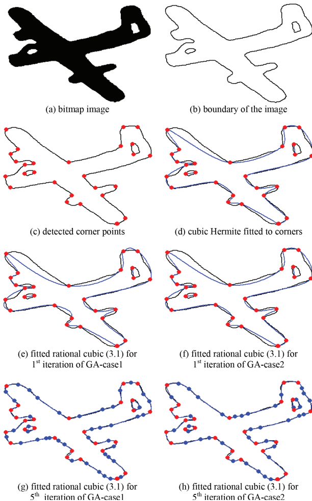
FIGURE 7. Demonstration of rational cubic function (3.1) using GA for case1 and case 2
