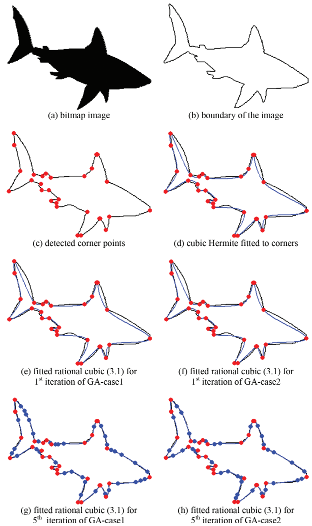
FIGURE 9. Demonstration of rational cubic function (3.1) using GA for case1 and case 2
