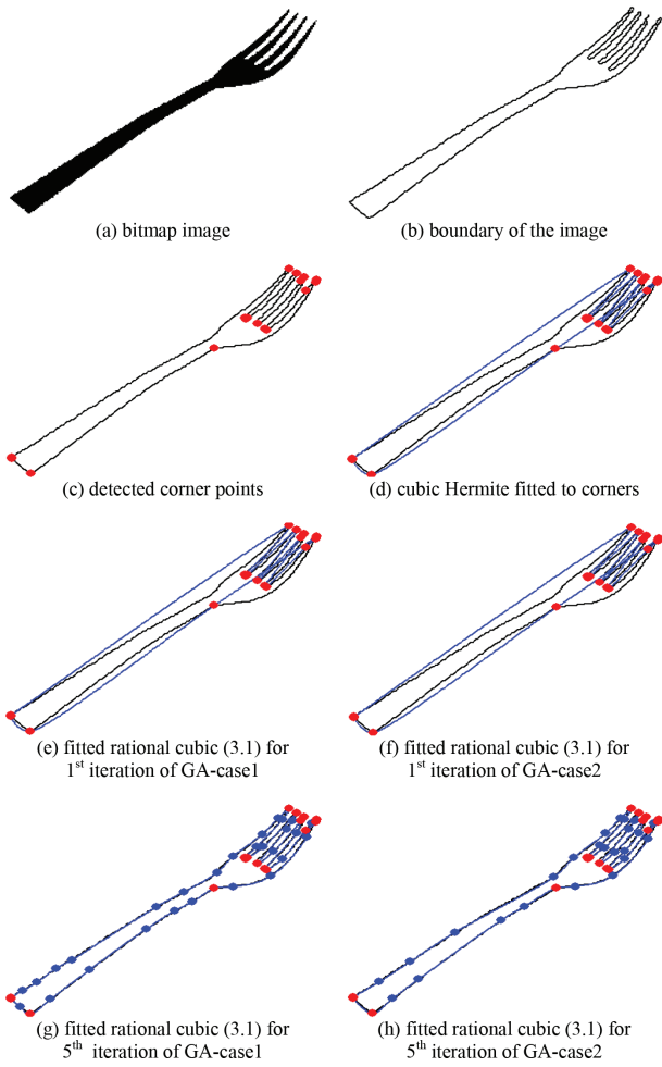
FIGURE 8. Demonstration of rational cubic function (3.1) using GA for case1 and case 2
