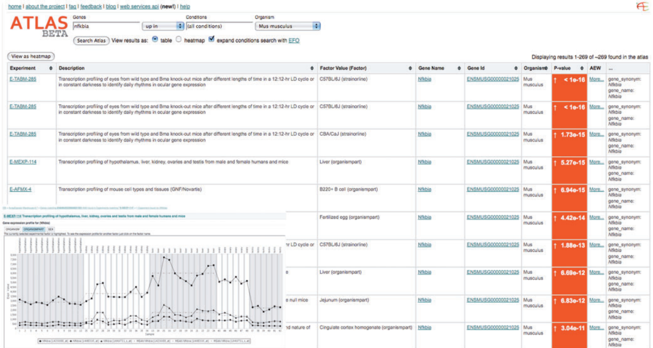
Figure 1. Table view from the ArrayExpress Atlas showing a query for up-regulation of the mouse gene Nfkbia in different experimental conditions. Columns from left to right: ArrayExpress experiment accession, experiment description, condition (factor value), gene name (linked to a gene view page), gene identifier, organism, P-value with an up/down indicator (red arrow for up, blue arrow for down) and a link to the ArrayExpress Warehouse for supporting data (inset bottom left).
