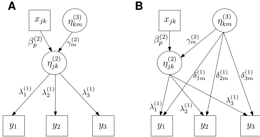
Figure 3: Graphical representation of Multilevel mixture ordinal item response models. Panel A shows a model that assumes complete measurement equivalence, panel B shows a model with country-item-bias effects \delta_{im}^{(1)}
