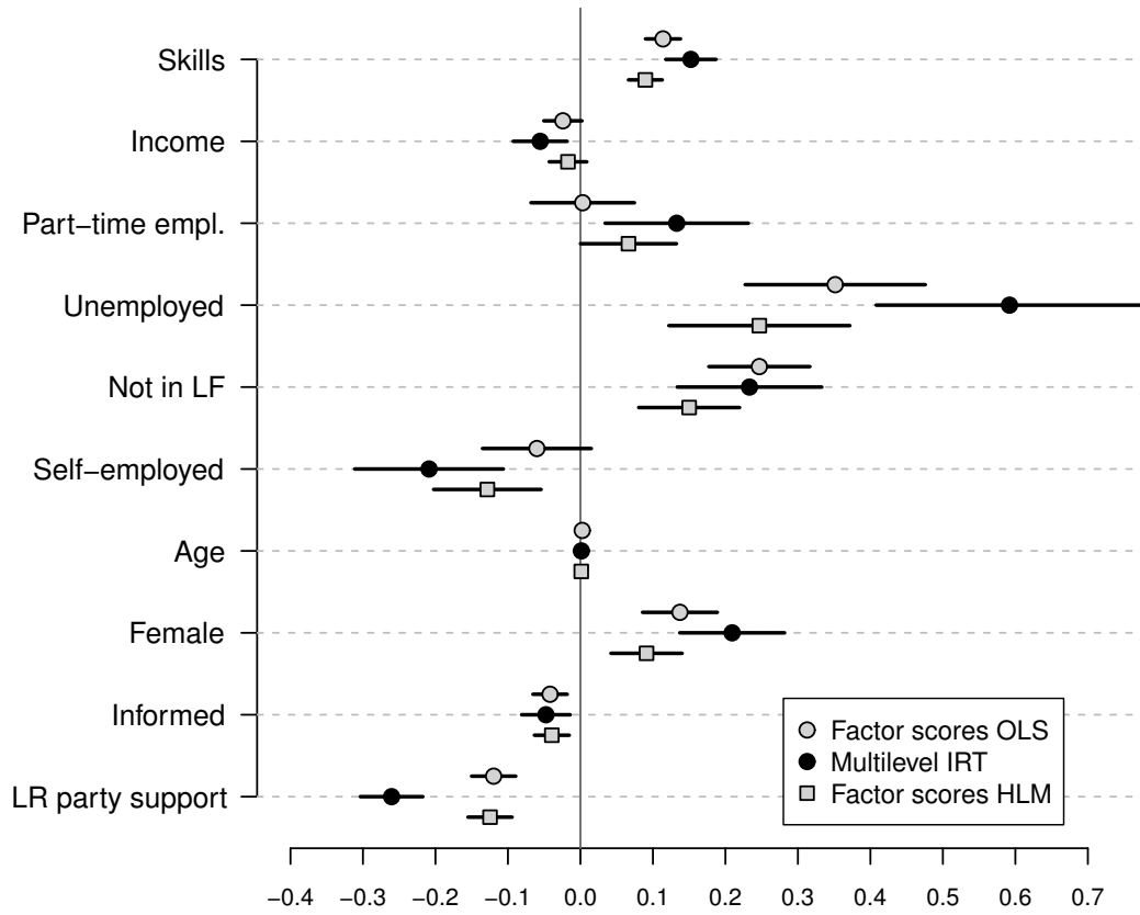
Figure 7: Point estimates and 95% confidence bounds for effects of covariates [\beta_p^{(2)}] on latent spending preferences from from Multilevel mixture ordinal item response model with item-bias effects (M4). Coefficients from a models using factor scores as dependent variable in a fixed-effects OLS regression with Huber-White standard errors and in a hierarchical linear model are shown for comparison.
