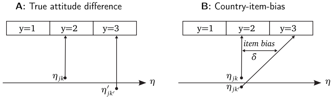
Figure 1: Ideal typical illustration of item bias. Panel A shows a situation where different responses of two individuals from different countries are the result of them having different preferences. Item-bias, as shown in panel B, exists when two individuals with the same preference give different responses simply because of country specific factors that influence their measurements.
