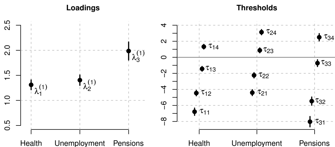
Figure 5: Point estimates and 95% confidence bounds for loadings [\lambda_i^{(1)}] and thresholds [\tau_{ic}] . Multilevel mixture ordinal item response model with item-bias effects (M4).
