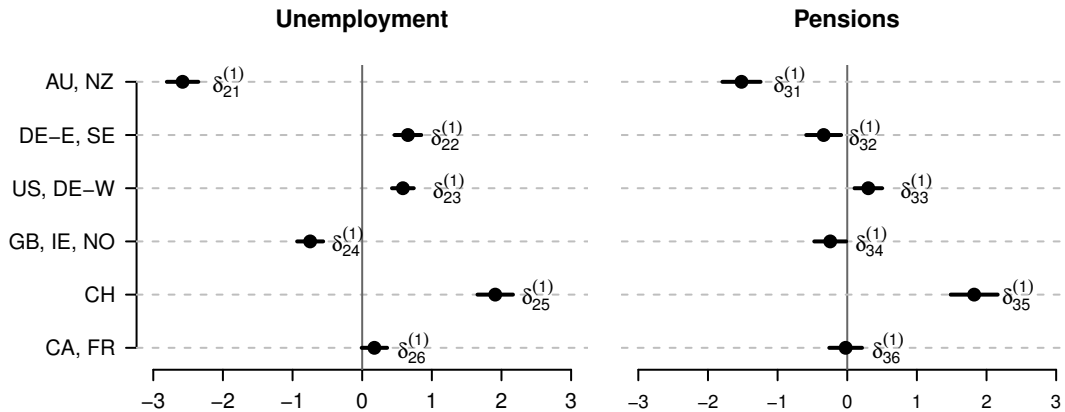
Figure 6: Point estimates and 95% confidence bounds for item-bias effects [ \delta_{im}^{(1)} ]. Multilevel mixture ordinal item response model (M4).
