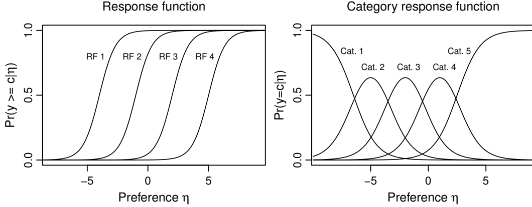
Figure 2: Illustrative response functions and associated category response functions for an item with parameters \lambda = 1.5 , \tau_1 = -4 , \tau_2 = -1 , \tau_3 = 2 , and \tau_4 = 5 .
