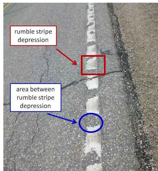
Figure 27. Wear at Vandalia/CR F70 after two years (Hallmark et al. 2011)
