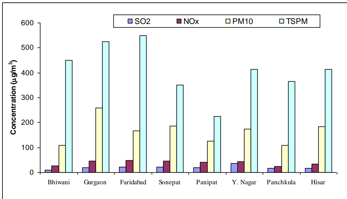
Fig 2: Average concentration of different pollutants ( \mu\text{g}/\text{m}^3 ) in different cities of Haryana
