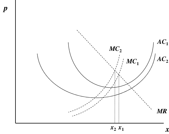
FigEx2c.pdf Figure 1: An Example of Submodularity
