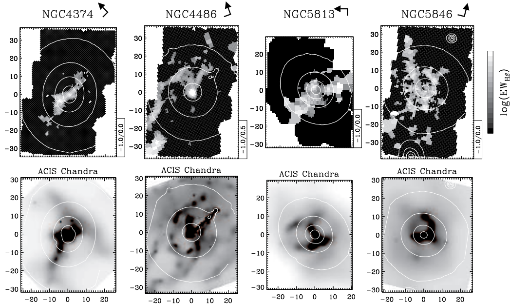
Fig. 3. Warm versus hot gas emission in four slowly-rotating SAURON galaxies. The top panels show the equivalent width of the H \beta line, in \text{\AA} and on a logarithmic scale, whereas the lower panels show smoothed maps for the X-ray emission observed with Chandra, in arbitrary units. Except in only few regions, nebular emission is usually associated to X-ray emitting features. For NGC 4486 and NGC 5846, this connection was already discussed by Sparks et al. (2004) and Trinchieri & Goudfrooij (2002), respectively
