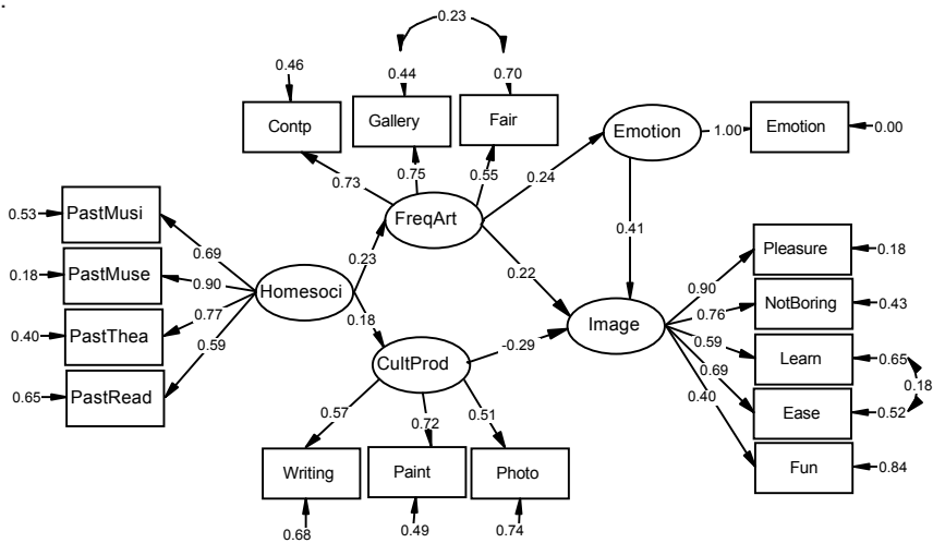
Figure 3. Path diagram of the selected structural model Note: Contp = other places of art contemporary than galleries and museums. Ordinal WLS. Imputation of missing values n=1,598. Coefficients are standardized.
