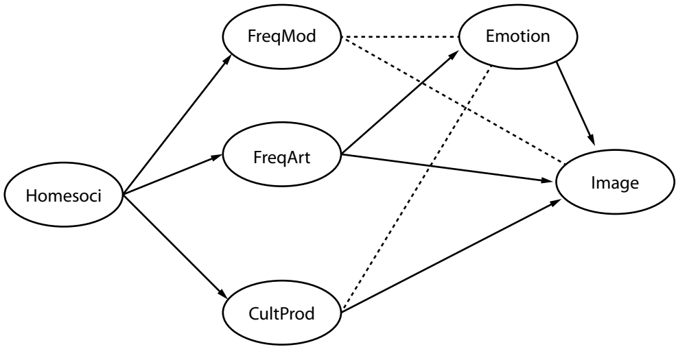
Figure 2. Conceptual diagram of the model Note: The hatched lines mean that the relation was not significant and was not kept in the final model.
