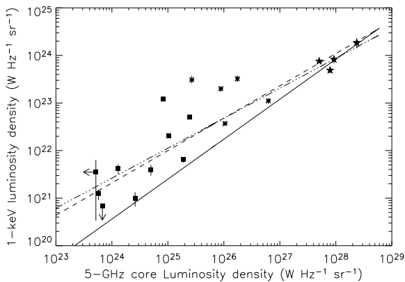
Figure 1. Luminosity-Luminosity relation. Filled boxes are RGs, asterisks are LDQs and star CDQs. Error bars show 1\sigma uncertainties. When these are not visible it is because errors are smaller than symbols. Upper limits are at the 3\sigma level. The continuous line is the best-fit regression to the sample of CDQs only. The dot-dashed line is the regression to the whole sample, while the dashed line fits the sample composed of CDQs and RGs
