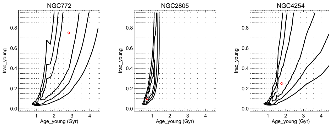
Figure 18. Contours of \Delta\chi^2 projected on the plane (age, fraction) of the young component at the 1,2,3- \sigma confidence level, for the central apertures of NGC 772, NGC 2805, NGC 4254; the red symbol marks the best-fitting model. These plots clearly show that the two-SSP approach is unable to constrain the fitted parameters, and that age and mass fraction of the young component are degenerate.
