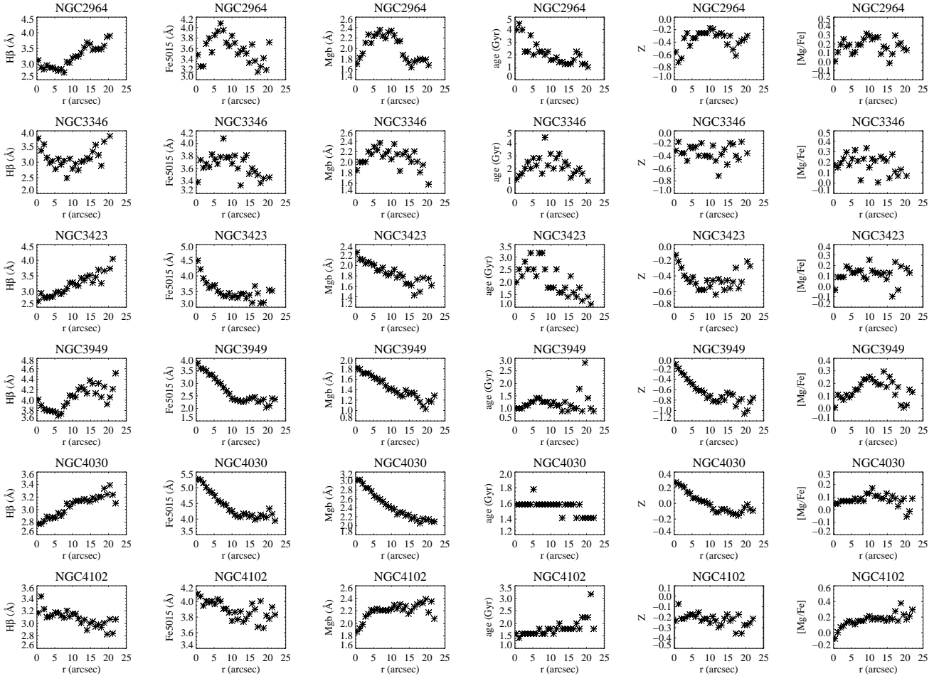
Figure A1b. Same as Figure A1a for NGC 2964, NGC 3346, NGC 3423, NGC 3949, NGC 4030 and NGC 4102.
