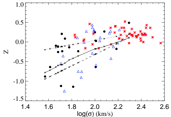
Figure 13. Relation between central metallicity and central velocity dispersion (in decimal logarithm and units of \text{km s}^{-1} ) for the E and S0 galaxies (Kuntschner et al., in preparation, red symbols) and the Sa (Paper XI, blue symbols) of the SAURON survey and for our late-type spirals (black dots), from our one-SSP analysis. The overplotted lines represent the relation metallicity - velocity dispersion obtained in different ways, drawn on the \sigma range of our data only: the dotted line reproduces Equation 6 (‘model approach’), the dashed line Equation 8 (‘empirical approach’) and the solid lines represents a relation based on the assumption of a set of index - \sigma relations. See text for a more complete description.
