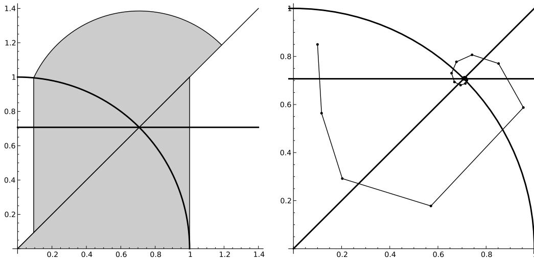
Figure 5: The picture in the left shows the regions of convergence in Theorem 2.1 for the Douglas-Rachford algorithm. The picture in the right illustrates an example of a convergent sequence generated by the algorithm.
