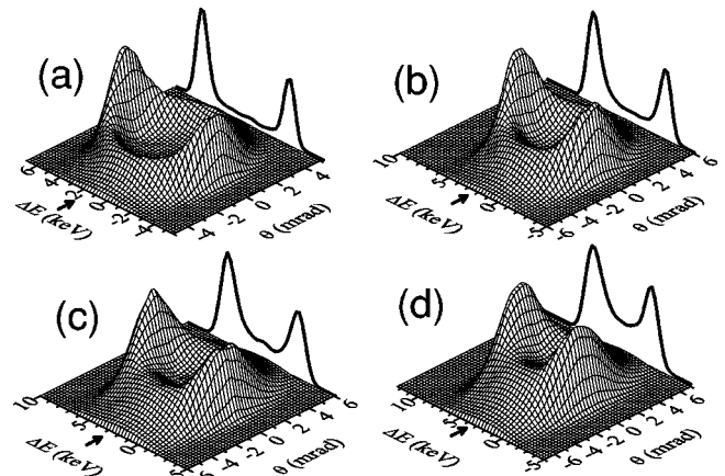
FIG. 3. Joint distribution of exit angle and energy loss of the fragment protons resulting from the dissociation of H_2^+ molecules of velocity v=5 a.u. after traversing amorphous carbon foils of several thicknesses D : (a) D=300 a.u., (b) D=500 a.u., (c) D=750 a.u., and (d) D=1000 a.u. The thick curves represent the energy-loss distribution at zero exit angle, whose mean value is indicated by an arrow.
