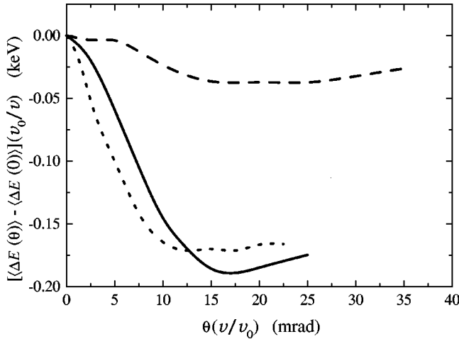
FIG. 5. Mean energy loss of proton fragments, relative to the mean energy loss at zero angle, as a function of their exit angle for a 150 a.u. thick amorphous carbon foil. We have scaled the energy-loss axis by v_0/v and the exit-angle axis by v/v_0 , where v_0 = 1 a.u. is the Bohr velocity. The dashed line corresponds to v = 1 a.u., the solid line to v = 2 a.u., and the dotted line to v = 5 a.u.
