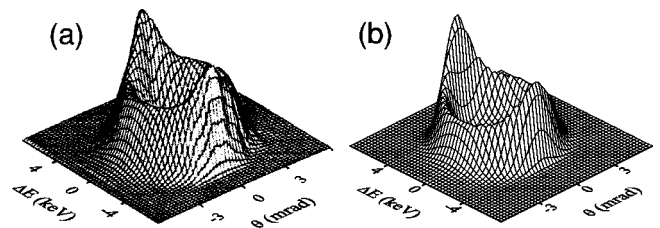
FIG. 4. Comparison between (a) the experimental [8] and (b) the calculated joint distribution of energy loss and exit angle of the fragment protons resulting from the dissociation of v=5.29 H_2^+ molecules in a 166 a.u. thick carbon foil. The experimental figure is reprinted with permission of the American Chemical Society.
