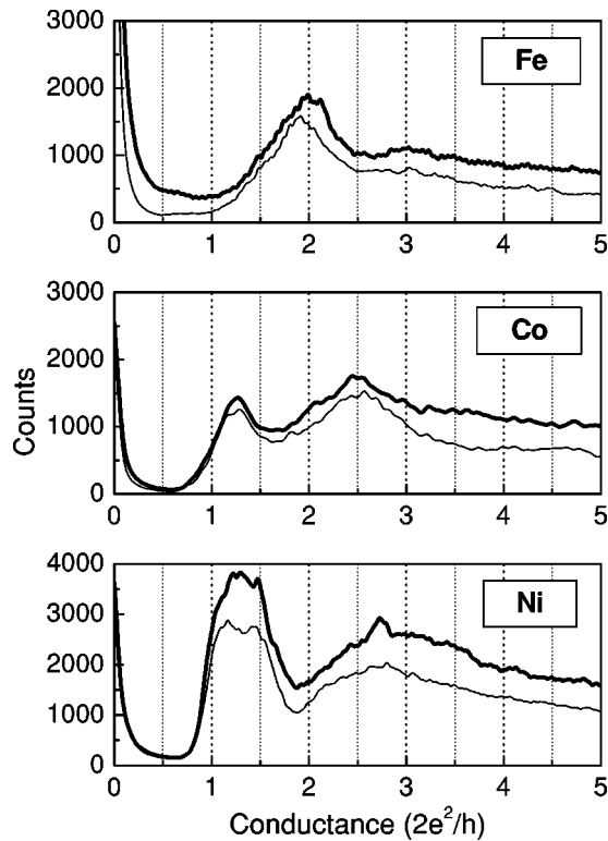
FIG. 1. Conductance histograms for the various metals without magnetic field (thin curve) and when a magnetic field of 5 T was applied (thick curve). The same structure was observed for every histogram recorded on different samples for the same metals. The conductance was measured using a dc bias voltage of 20 mV, and the histograms were constructed using 2500 traces (Fe), 1500 (Co and Ni at 5 T) or 3000 traces (Ni at 0 T).
