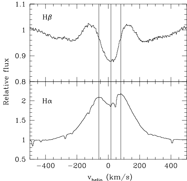
Fig. 1. The spectrum around H\alpha and H\beta . The vertical lines are drawn through the H\alpha peaks and the systemic velocity. The larger peak separation in H\beta suggests that the hydrogen recombination lines are formed in a rotating Keplerian type disk.
