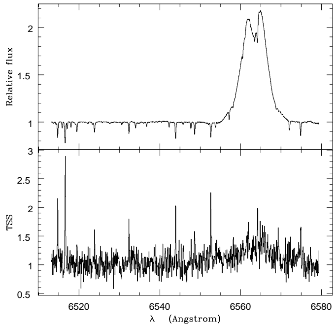
Fig. 3. Top panel: The continuum corrected total spectrum of the echelle order covering H\alpha . Lower panel: TSS spectrum in the H\alpha order. The telluric absorption lines again show up as healthy variable lines, across the H\alpha line the variations are marginal.
