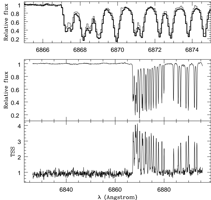
Fig. 2. The spectrum around the telluric lines at 6860 \text{ \AA} . The upper panel shows part of the spectrum, where the thick line represents the last spectrum taken and the thin line the first spectrum, obtained almost two hours earlier. It is clear that the telluric absorption has become stronger. The middle panel shows the total, continuum rectified, spectrum, and the lower panel presents the TSS. While the continuum does not show any significant variations, the changes in the telluric lines show up as strong peaks in the TSS.
