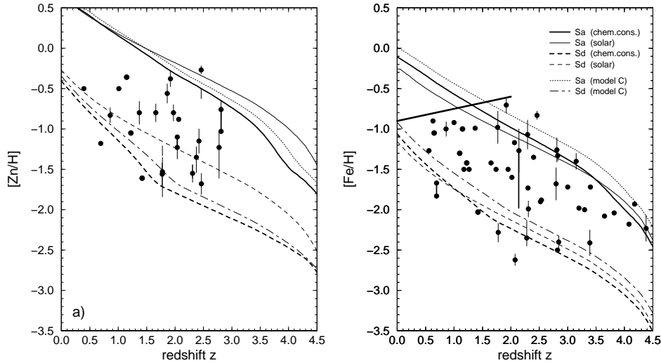
Figure 1. Redshift evolution of [Zn/H] (1a) and [Fe/H] (1b) for models Sa and Sd compared to observed DLA abundances.
