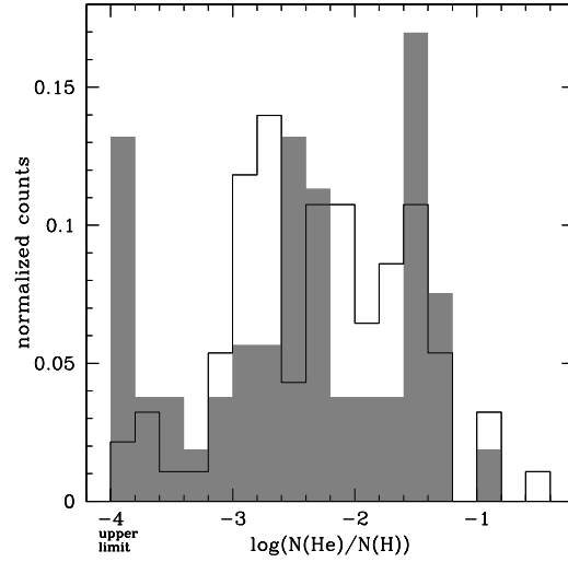
Figure 2. Shaded histogram: Helium abundance distribution of our sdB stars. Open histogram: Distribution from Edlmann et al. (2003).
