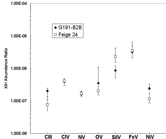
Figure 7. Comparison of measured abundances for Feige 24 and G191-B2B.
