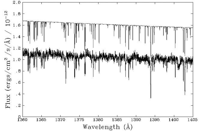
Figure 3. 1360Å to 1405Å region of the STIS spectrum of REJ0558-373, showing photospheric lines of Ov (1371.296Å), Siiv (1393.755/1402.770Å) and Fev. The best-fit synthetic spectrum is shown offset for clarity.
