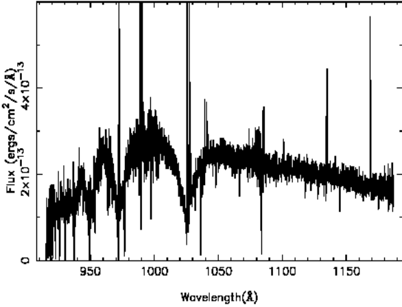
Figure 1. Composite FUSE spectrum of the hot DA white dwarf PG1342+444 produced by co-adding the individual exposures and merging the resulting spectra for the individual detector segments.
