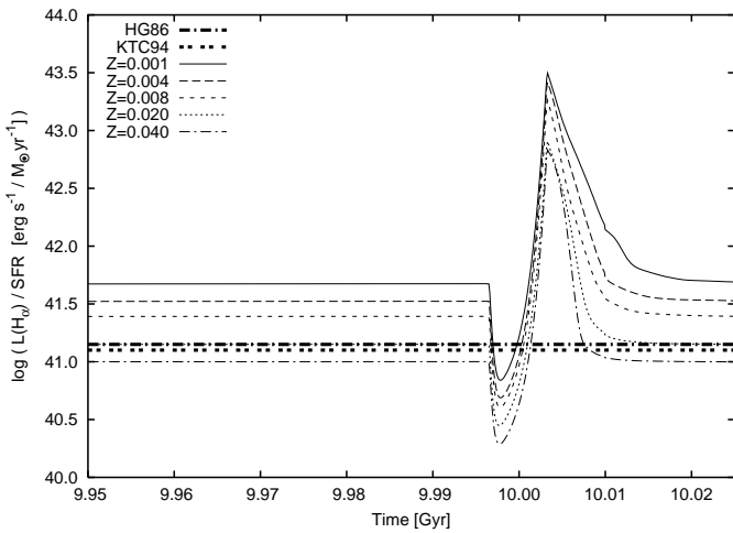
Fig. 2. \nu^2 = L(H_\alpha) / \text{SFR} over time for Gaussian bursts with short timescale of \tau_B = 10^6 yr.
