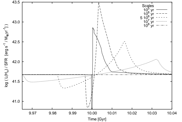
Fig. 3. \nu^2 = L(H_\alpha) / \text{SFR} over time for Gaussian bursts with different timescales and Z = 0.001 .
