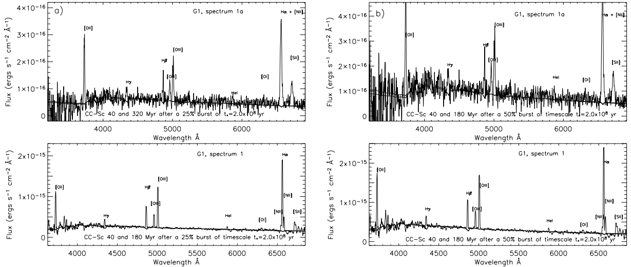
Fig. 3. a) CC-Sc model spectra calculated 40 (thick line) and 180 or 320 (thin lines) Myr after a 25% burst compared with the two spectra of G1 at PA 90^\circ (top) and 130^\circ (bottom) after internal reddening correction (see text). The reduced- \chi^2 is in the range 0.12–0.16 (however, see discussion in Sect. 3). b) Same as a) for a model with a 50% burst. Model spectra at both burst ages acceptably reproduce the observed spectra. A minimum reduced \chi^2 = 0.12 is obtained for both spectra at age 180 Myr, while the 40 Myr model gives a reduced \chi^2 = 0.16 and 0.15 for spectra 1a and 1, respectively.
