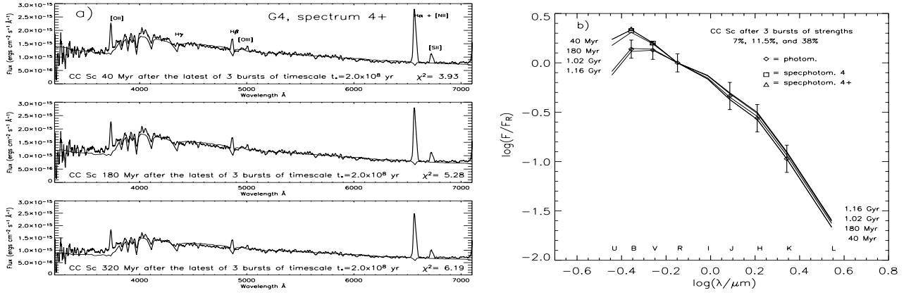
Fig. 15. a) Spectrum of G4 at PA 90^\circ corrected for internal reddening and overlapped with CC-Sc model spectra (thick line) at three different ages after the latest of three interaction-induced bursts of star-formation (see text). b) SED for the CC-Sc model at three ages after the latest of three interaction induced bursts. Photometric points of G4 are marked with diamonds, while the spectrophotometric points derived from the dereddened spectra at PA 130^\circ and 90^\circ are indicated by triangles and squares, respectively. The thick line indicates the best fit age, according to the spectral analysis.
