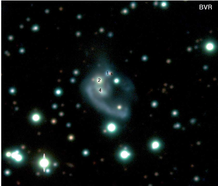
Fig. 1. BVR composite image of CG J1720-67.8. Numbers indicate the three main galaxies, while the “s” label indicates an M-type foreground star seen in projection on G1. North is on top, east to the left. The size of the field is \sim 2'.3 \times 1'.9 . At the distance of the group, 1'' \sim 0.9 kpc.
