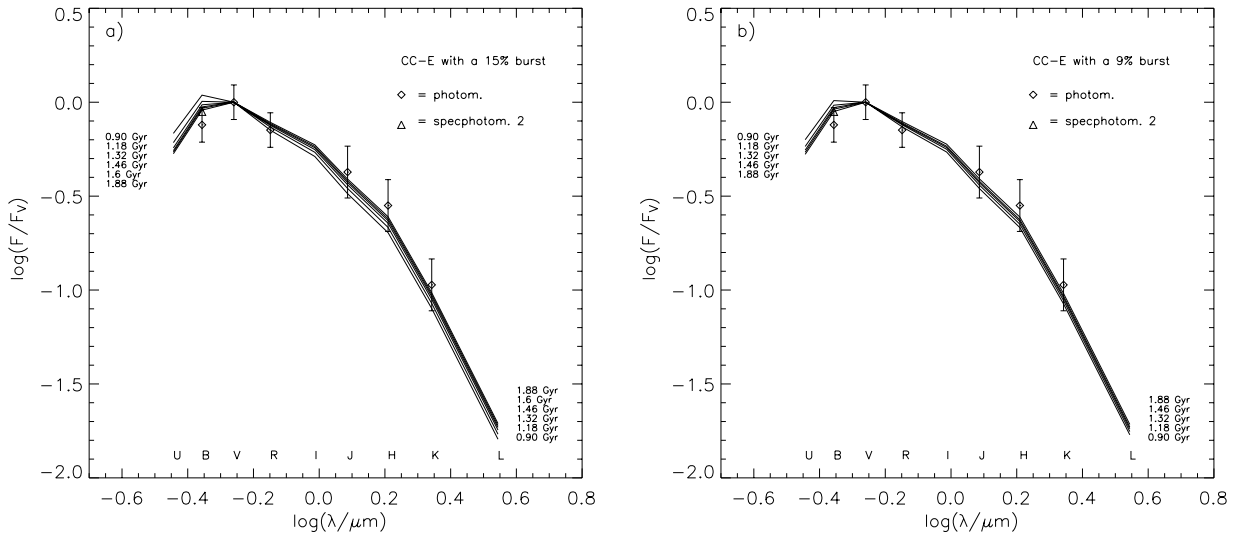
Fig. 13. SEDs for the CC-E models with burst strength 15% ( left ) and 9% ( right ), along with dereddened photometric (diamonds) and spectrophotometric (triangle) data points for G2. Best-fit ages according to the spectral analysis are indicated with a thick line. Discrepancies are visible in the NIR.
