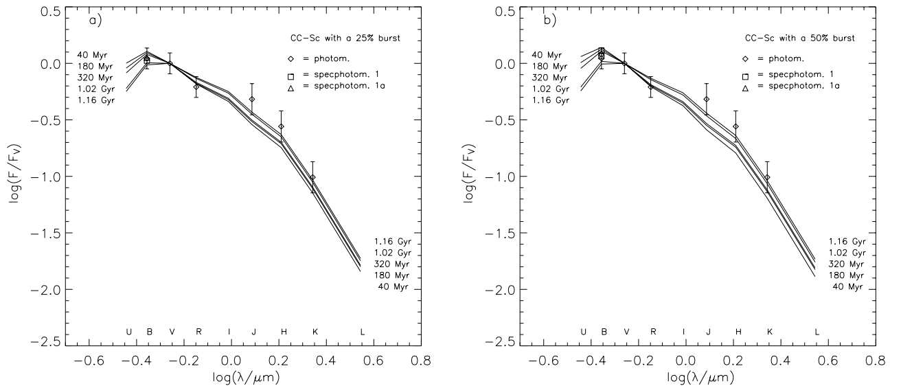
Fig. 6. Energy distribution normalized to the V band for CC-Sc models in a wide range of burst ages after the onset of a 25% [a)] and a 50% [b)] burst. Diamonds with associated error bars are photometric observational points for G1, after correction for inclination. The square and the triangle are spectrophotometric points obtained from the observed, dereddened, spectra 1 and 1a after convolution with B and V filter response functions (Bessell 1990).
