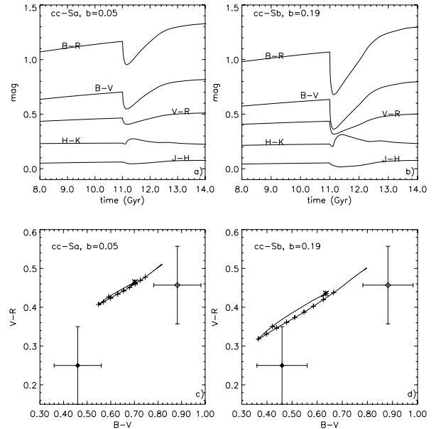
Fig. 8. a) Evolution of color indices for a cc-Sa model with a 5% burst switched on after 11 Gyr of undisturbed evolution. The B - V index is indicated with a thick line to avoid confusion with other indices. For the same reason, an offset of -0.5 was applied to the J - H index. b) Same as a) , for cc-Sb model with a 19% burst. c) Color-color diagram showing the color indices evolution during the burst phase for a cc-Sa model with a 5% burst. The asterisk marks the onset of the burst at a galaxy age of 11 Gyr. Plus symbols are plotted for burst ages from 40 Myr to 1.28 Gyr at intervals of 140 Myr. The empty diamond indicates the observed colors of G2, after a standard inclination correction. The full diamond indicates the observed colors after correction for internal extinction using E(B - V)_g = 0.52 mag, as derived from the Balmer decrement. d) Same as c) for a cc-Sb model with a 19% burst.
