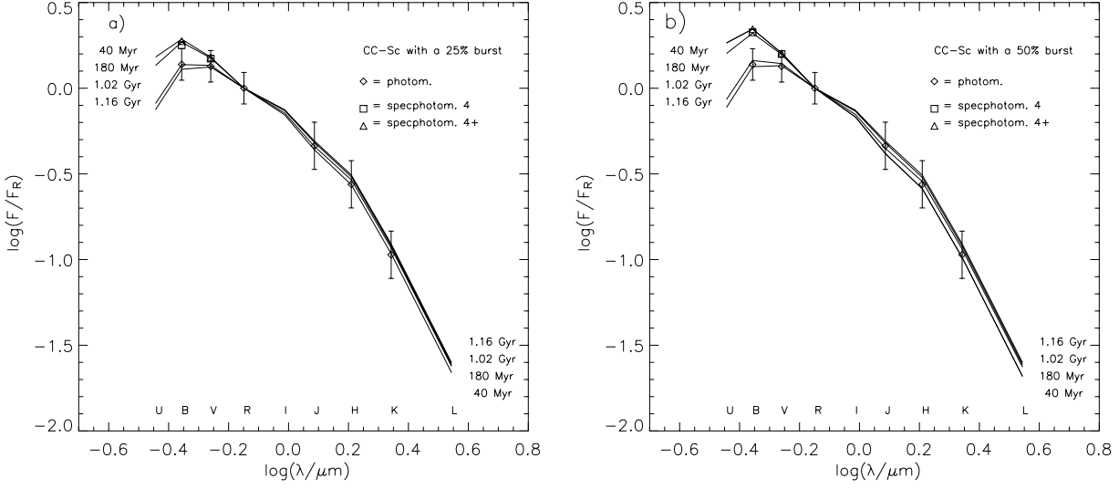
Fig. 7. SEDs for the CC-Sc models at differing ages after a weak [a)] and a strong [b)] burst. Photometric points of G4 are marked with diamonds, while the spectrophotometric points derived from the dereddened spectra (according to the best-fit extinction values obtained from the spectral analysis) at PA 130° and 90° are indicated by triangles and squares, respectively. For models of both strengths, optical spectrophotometric points and NIR photometric points agree very well with a burst age in the range 40 to 180 Myr. The thick line indicates the best-fit age obtained from the spectra.
