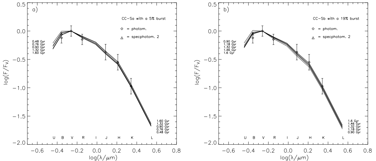
Fig. 10. SEDs calculated for a wide range of burst ages for the CC-Sa [a)] and Sb [b)] models, along with dereddened photometric and spectrophotometric data points for G2. The thick lines indicate the best-fit models according to the spectral analysis.
