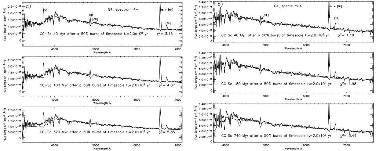
Fig. 5. a) CC-Sc model spectra calculated 40, 180, and 320 Myr (from top to bottom, thick line) after a 50% burst compared with the spectrum of G4 at PA = 90°, after internal reddening correction (see text). Reduced- \chi^2 values are indicated. The first two models are in good agreement with the data, while the third one departs from the observations in the blue part of the spectrum. b) Same model as in a) compared to the spectrum of G4 at PA = 130° for burst ages 40, 180, and 740 Myr. Reduced- \chi^2 values are marked. The older burst model departs from the observations significantly, while the first two models match the data reasonably well.
