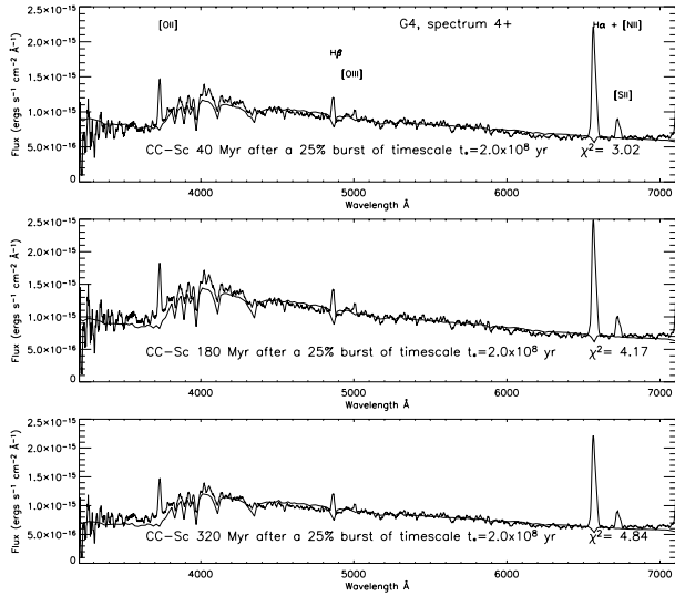
Fig. 4. CC-Sc model spectra calculated 40, 180, and 320 Myr (from top to bottom, thick line) after a 25% burst compared with the spectrum of G4 (at PA = 90°) after internal reddening correction (see text). The reduced- \chi^2 of the fit for the 3 model ages based on continuum intervals and absorption line equivalent widths, minimized over a range of possible internal extinction values, is indicated.
