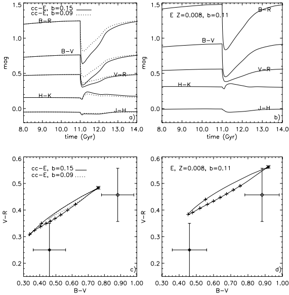
Fig. 11. a) Evolution of color indices for a CC-E model with a 15% (solid line) and a 9% (dotted line) burst switched on after 11 Gyr of undisturbed evolution. The B - V index is indicated with a thick line to avoid confusion with other indices. For the same reason, an offset of -0.6 has been applied to the J - H index. b) Same as a) , for a non-CC E model with metallicity Z = 0.008 and a 11% burst. c) Color-color diagram showing the evolution of the color indices during the burst phase for the CC-E model. Line styles are as in a) . Symbols as in Fig. 8. d) Same as c) for the non-CC E model.
