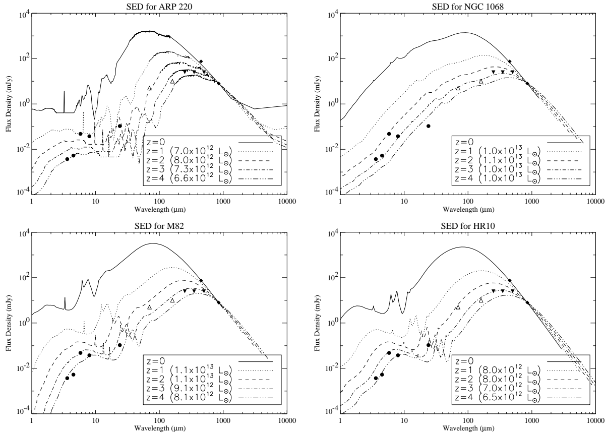
Figure 1. Model spectral energy distribution plots of template galaxies with survey sensitivities overplotted. Filled circles : SWIRE sensitivities 500 seconds, 5\sigma (Lonsdale et al. 2004). Open triangles : The pre-flight Spitzer sensitivities for 70 and 160 \mu\text{m} are shown whilst the SWIRE team re-assess their observing strategy due to the degraded MIPs sensitivities, although currently these are expected to be two to three times worse. Filled triangles : The pre-flight BLAST confusion limit estimates (derived from Rowan-Robinson 2001) of 25 mJy; the sensitivity estimates (Hughes et al. 2002) are in the range 15 – 25 mJy. Filled diamonds : SHADES survey sensitivities of 8 mJy at 850 \mu\text{m} and 75 mJy at 450 \mu\text{m} . Models have been normalised to the SHADES survey depth of 8 mJy at 850 \mu\text{m} . Top left panel : Arp 220 – a highly-obscured local starburst galaxy (note: it is also a ULIRG Elbaz et al. 2002). Top right panel : NGC1068 – a typical Seyfert galaxy (Efsthathiou, Hough & Young 1995). Bottom left panel : M82 – an irregular dusty star-forming galaxy (Efsthathiou, Rowan-Robinson & Siebenmorgen 2000). Bottom right panel : HR10 – a high-redshift, extremely-red galaxy (Takagi, Hanami & Arimoto 2004). Bolometric (3–1000 \mu\text{m} rest-frame) luminosities for each model, as normalised, are shown in the legends.
