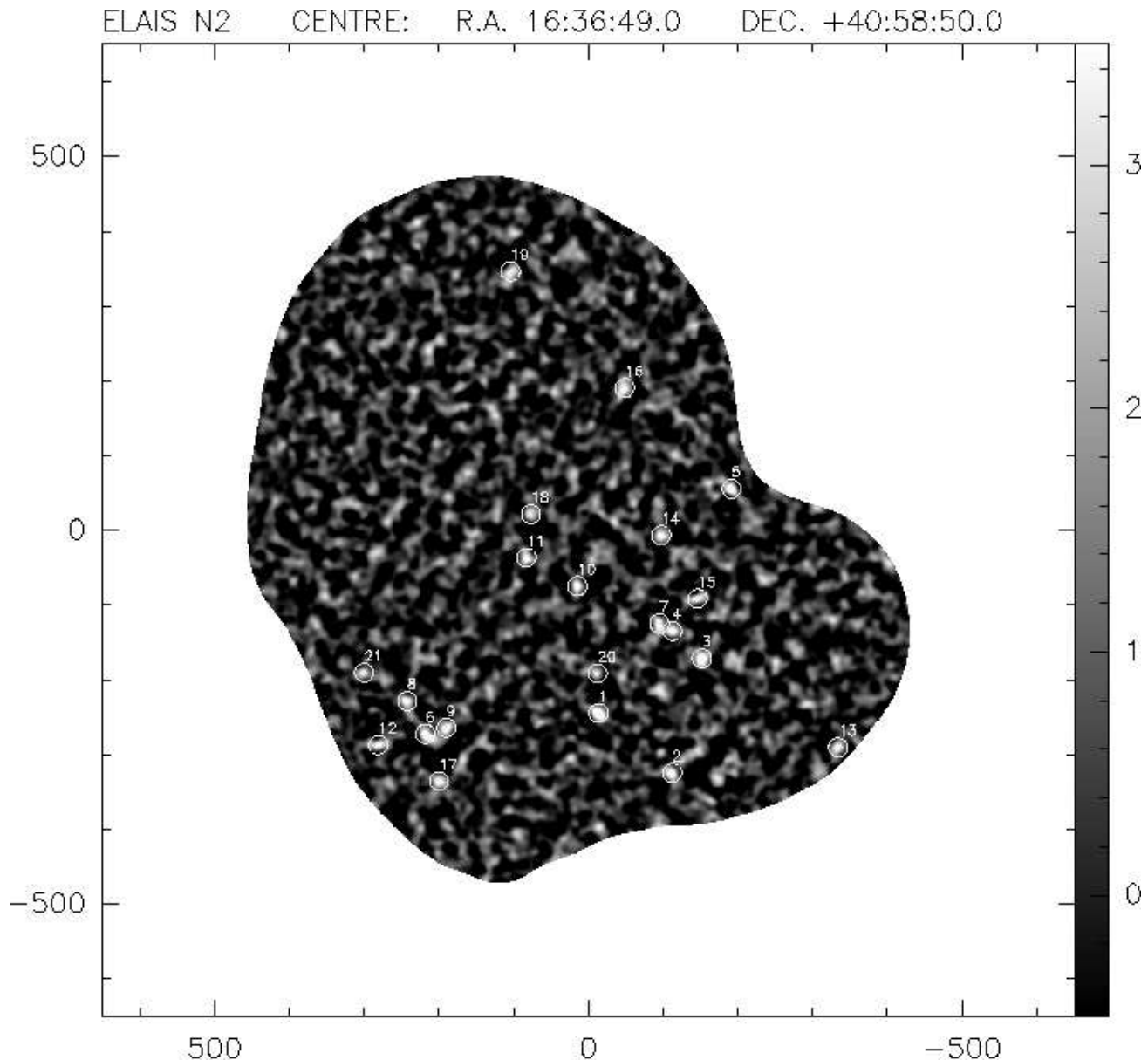
Figure 3. 1200 \mu\text{m} MAMBO signal-to-noise map of the ELAIS N2 field. Sources detected at \geq 3.5\sigma are circled in white, and are numbered in order of significance. The axes denote the offset (arcsec) from the map centre.
