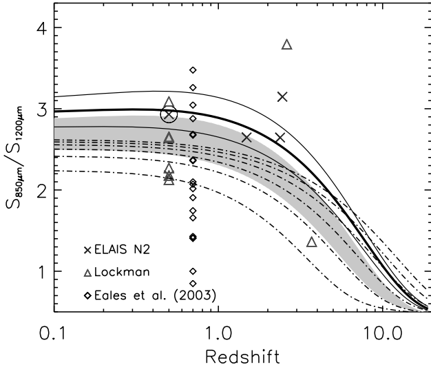
Figure 13. The 850/1200 \mu\text{m} flux density ratio for SCUBA sources detected by MAMBO in the ELAIS N2 (crosses) and Lockman Hole (triangles). Six of the sources have spectroscopic redshifts (see Chapman et al. 2003, 2004), while the remainder have been placed at z = 0.5 . The two encircled sources have no radio counterpart. Shown as diamonds are the 850/1200 \mu\text{m} flux ratios for the sample of Eales et al. (2003). The thick solid curve represents the expected flux ratio for an optically thin modified blackbody with T_d = 45 K and \beta = +1.5 , typical for a local ULIRG. This curve is enveloped by two thin solid curves which correspond to changes in the dust temperature and spectral index of \Delta T_d = \pm 5 K and \Delta\beta = \pm 0.2 . The light-grey shaded area corresponds to a modified blackbody with T_d = (35.6 \pm 5.0) K and \beta = (+1.3 \pm 0.2) . The dot-dashed curves corresponds to SEDs with \beta = 1.0 and T_d = 20\dots 70 K in step of 10 K.
