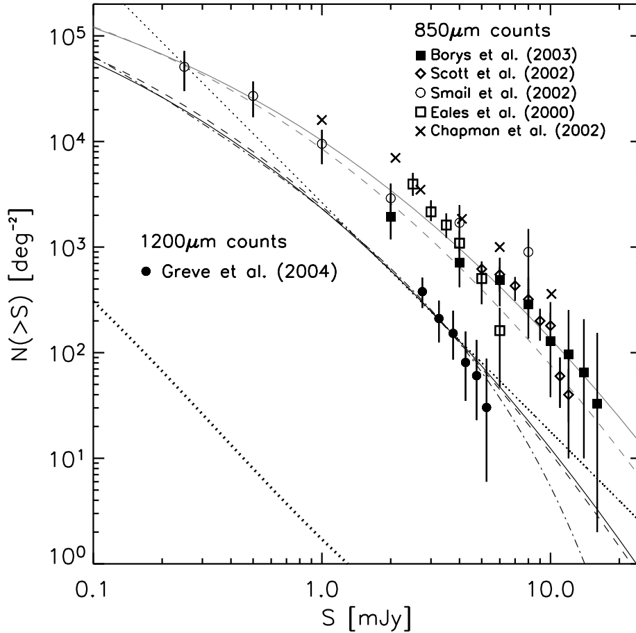
Figure 7. Cumulative number counts at 1200\mu\text{m} (solid circles) based on the \geq 3.5\sigma MAMBO source catalogue presented in this paper. The error bars represent 95 per cent two-sided confidence levels on a Poissonian distribution. Also shown are 850\mu\text{m} cumulative number counts from a number of recent SCUBA surveys. The dashed black and grey lines show the number counts at 1200 and 850\mu\text{m} , respectively, as predicted by a pure luminosity scenario in which g(z) = (1+z)^3 out to z = 2 , beyond which no further evolution occurs. The solid black and grey curves represent predicted number counts at 1200 and 850\mu\text{m} , respectively, based on the galaxy evolution model by Jameson et al. (1999), see text for details. The thin dotted line corresponds to a simple power law with slope \alpha = -2.2 , while the dark solid curve represents the Schechter function dN/dS \propto (S/S_0)^{-\alpha} \exp(-S/S_0) , where \alpha = 2.3 and S_0 = 4 \text{ mJy} . Finally, the thick dotted line represent a no-evolution scenario.
