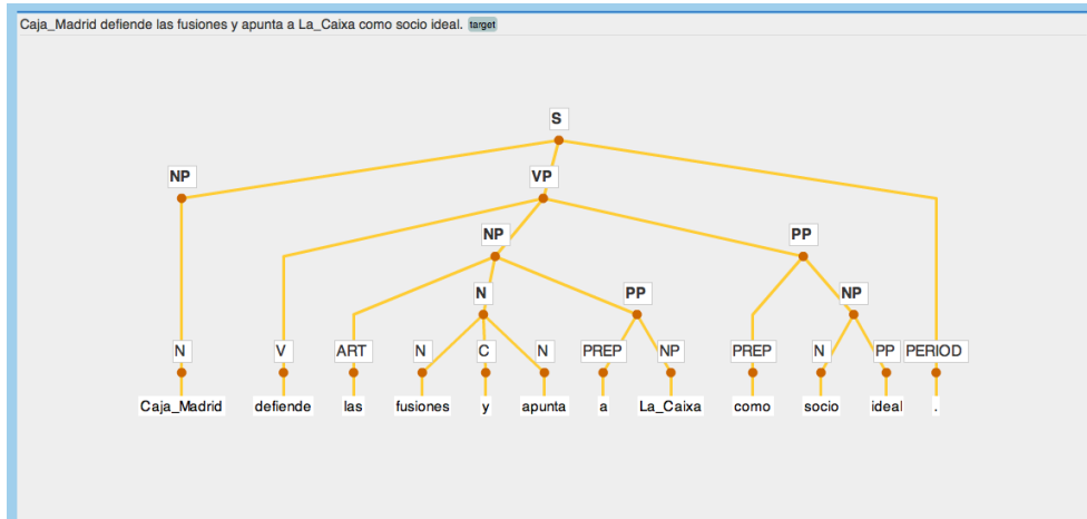
(a) System: Output tree #1
