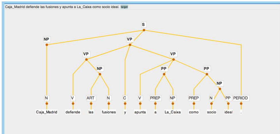
(c) System: Output tree #2
