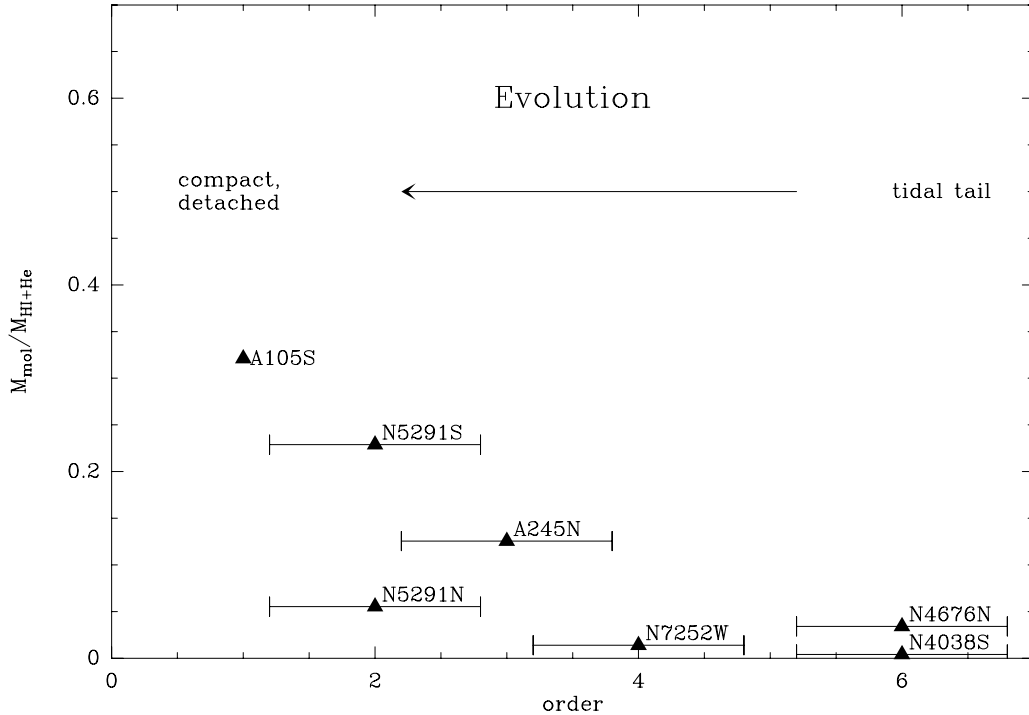
Fig. 9. Comparison of the \text{H}_2/\text{HI} mass ratio with the evolutionary order of the TDGs. NGC 7319E was not included due to its unclear morphology (see Fig. 6). The single non-detection, IC 1182E, was also left out. The errorbars indicate the uncertainty in the evolutionary order based on the criteria described in the text. The source names are to the right of their positions.
