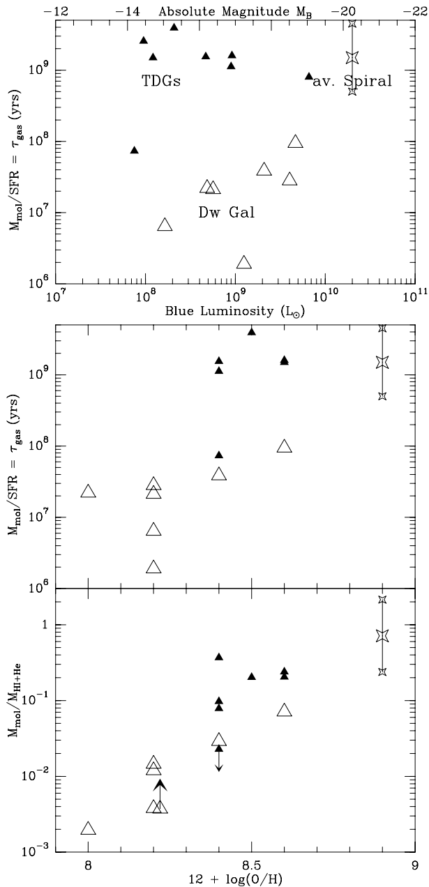
Fig. 8. (Top): comparison of gas consumption time, M_{\text{mol}}/\text{SFR} , which is the inverse of the frequently used Star Formation Efficiency (SFE), as a function of blue luminosity for the different categories of galaxies. Small filled triangles represent the TDGs (data from Tables 2 and 5), open triangles the regular dwarf galaxies (data from Table 4), and the star an average spiral as taken from Kennicutt (1998), similar in position on the diagram to the Milky Way. For Arp 245N values are for the CO-detected area, not just the center. The smaller stars give the range for “average” spirals. (Middle): as above but as a function of oxygen abundance. (Bottom): molecular to atomic gas mass ratios as a function of oxygen abundance. NGC 4214 has been moved slightly to the right to make it visible and the up arrow is because the HI mass is for a substantially greater area than covered by the CO observations. The same N(\text{H}_2)/I_{\text{CO}} value has been used for all galaxies, irrespective of metallicity or other influences, so M_{\text{mol}} is likely underestimated by a varying factor for the non-TDG dwarf galaxies.
