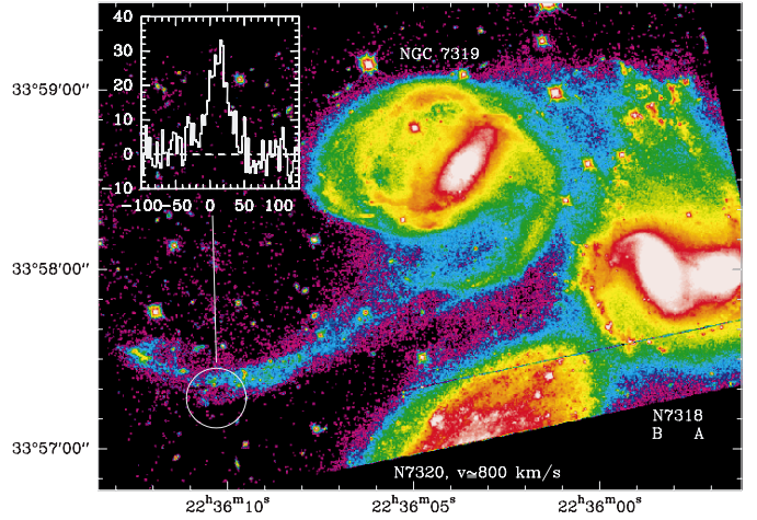
Fig. 6. Hubble Space Telescope V -band mosaic of Stephan’s Quintet. Spectrum is CO(1–0) emission and the circle marks the position observed in CO, which is the HI column density peak as observed by Shostak (1984). The zero velocity corresponds to cz = 6600 \text{ km s}^{-1} . NGC 7320 is a foreground galaxy.
