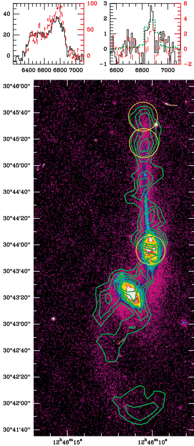
Fig. 5. The NGC 4676 “The Mice” system: R band image with green HI contours (Hibbard & van Gorkom 1996) superimposed. First HI contour and contour spacing is 2.5 \times 10^{20} \text{ cm}^{-2} ; the spatial resolution is 12'' . The circles mark the positions observed in CO and the TDG spectra are at the top right and the spectra of the center of NGC 4676a (Northern spiral) at the top left. The TDG CO spectra are the sum of the two positions towards the end of the tidal tail. The CO(2–1) spectra (red, dashed) follow the red right scale and the HI spectrum is in arbitrary units.
