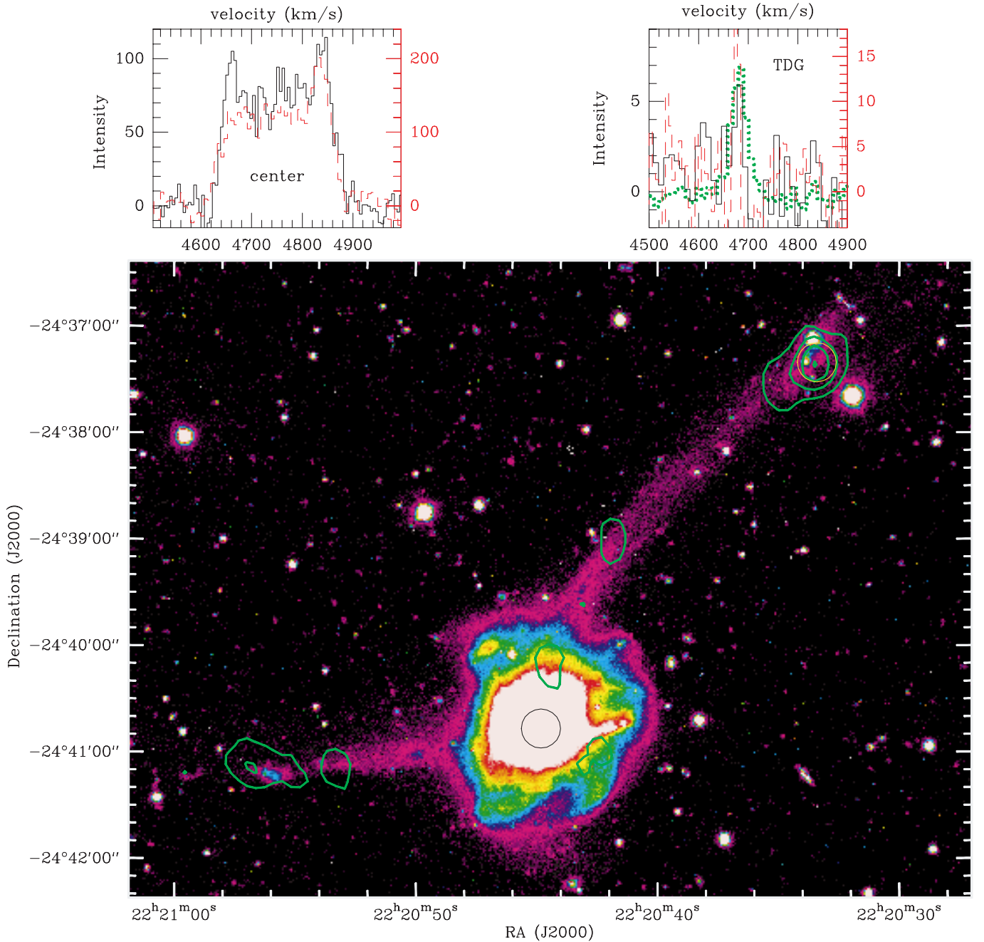
Fig. 1. V-band image of the NGC 7252 “Atoms For Peace” system with two tidal dwarfs, NGC 7252W and NGC 7252E, the latter of which was not observed in CO. The image is saturated to show the stars in the tidal tails. The green contours represent HI column densities (Hibbard & van Gorkom 1996) of 2, 3, 4, 5 \times 10^{20} \text{ cm}^{-2} at 27'' \times 16'' resolution. Circles show the positions observed in CO; the size of the circle is that of the CO(1–0) beam. Above the image the spectra of the Western TDG, NGC 7252W, and the center of the merger are shown and color coded as follows: HI as thick dotted green, CO(1–0) as black and CO(2–1) as dashed red. The velocities are in \text{kms}^{-1} and the left vertical scale gives the intensity in mJy per beam for the HI and mK for the CO(1–0). The right vertical scale indicates the CO(2–1) line strength in mK. CO observations are presented on the main beam temperature scale.
