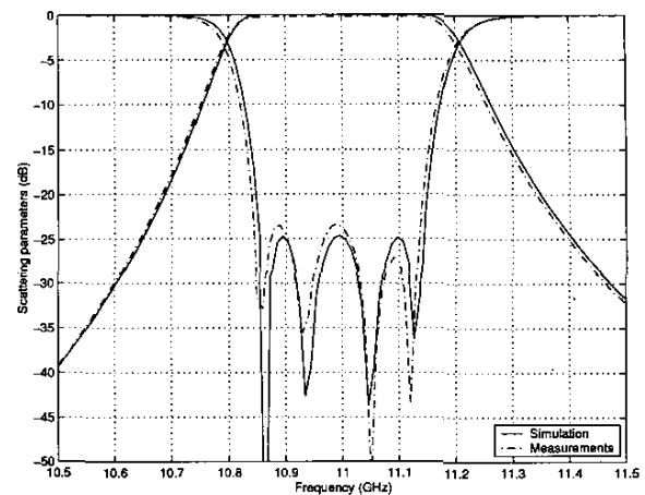
Fig. 6. Simulated and measured S-parameters of the four pole inductive filter with rounded corners.
