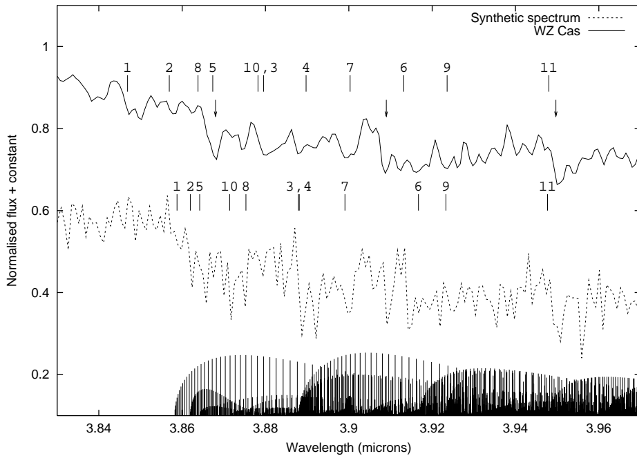
Figure 8. The observed spectrum of WZ Cas over the region of 3.8-4.0 \mu\text{m} , with a synthetic spectrum at T=2800\text{ K} , \log(N_{\text{C}}/N_{\text{O}}) of 0.003 and V_T = 3.5\text{ km s}^{-1} . A constant is subtracted from the flux of the synthetic spectrum to stagger it from the observed spectrum. The Q branch lines in this spectral region in the ab initio data of Harris et al. (2002b) are plotted at the bottom of the figure with line length in proportion to line intensity. The experimental band centres of the (0,1,1,0)\rightarrow(1,0,0,0) band and its hot bands are indicated by the upper series of marks and digits. Likewise the lower series of marks and digits identify the band centres of the ab initio data of Harris et al. (2002b). The downward pointing arrows indicate the position of CS band heads. The data for the HCN bands with their index is tabulated in table 3.
