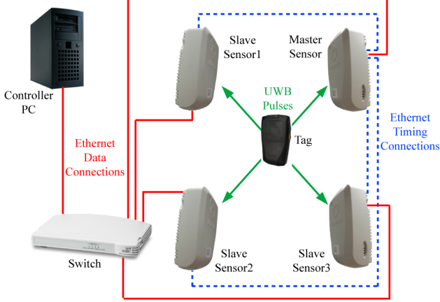
Figure 3. Ubisense architecture.
