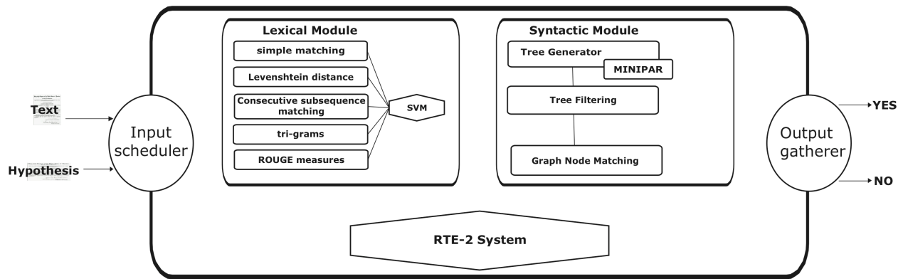
Figure 1: System architecture.
