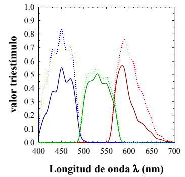
Figure 2: Pseudo-color matching functions for the RGB (dashed lines) UVW (solid lines) colorimeter.
