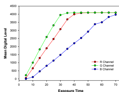
Figure 2: Mean digital level vs. exposure time for R, G and B channels for the QImaging RETIGA
