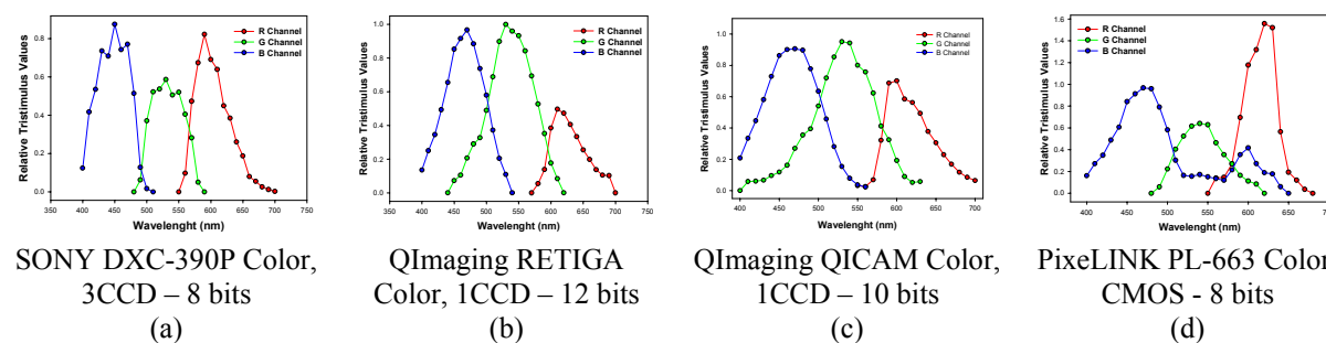
Figure 3: Color matching functions for (a) SONY DXC-390P Color, 3CCD – 8 bits, (b) QImaging RETIGA Color, 1CCD – 12 bits, (c) QImaging QICAM Color, 1CCD – 10 bits and (d) PixeLINK PL-663 Color, CMOS - 8 bits.
