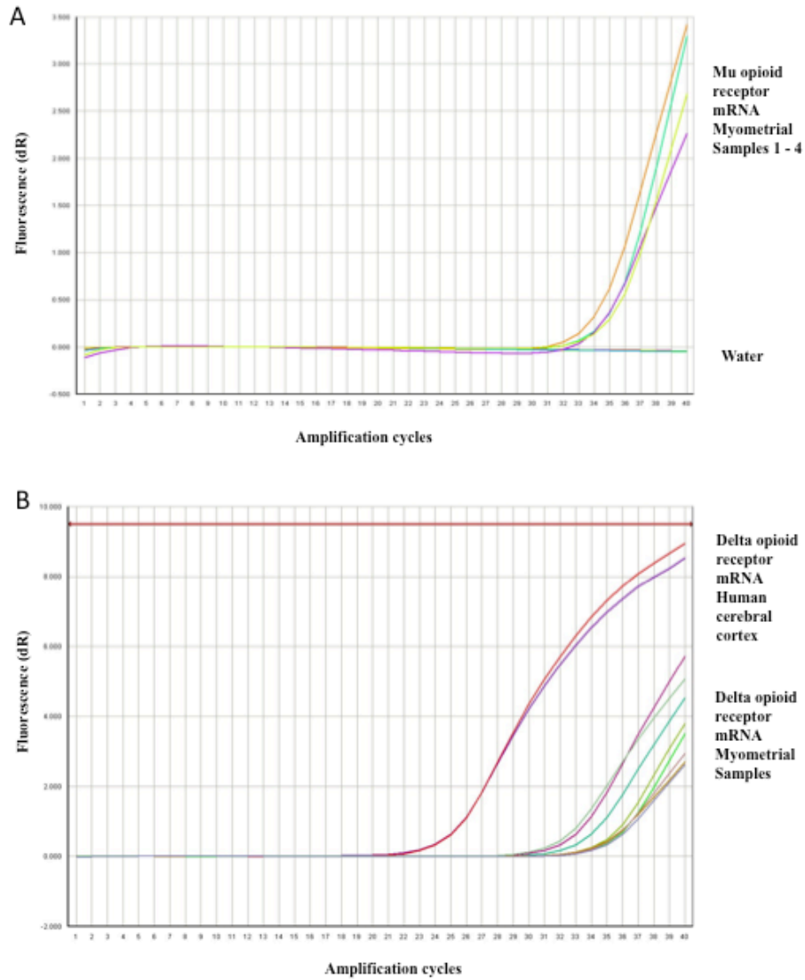
Fig. 2. Real-time PCR curves from the inner myometrial layer of the lower uterine segment of human term pregnant uterus for (A) mu and (B) delta opioid receptors (OR). A deflection before the 35th cycle of amplification was considered significant. Mu and delta OR Ct values were normalised relative to the amount of constitutively expressed GAPDH and normalised Ct values plotted. The mean Ct value for mu was 34.09 and for delta was 32.99.
