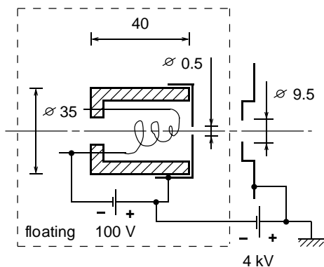
Figure 4.3.: Plasma ion source: The body of the source is machined in BN_3 ceramics. From the discharge between the filament and the anode positive ions are extracted through the hole in the anode. Through the larger hole from the left a charge holder with a compound containing the desired atoms can be inserted. The approximate dimensions are given in mm.
