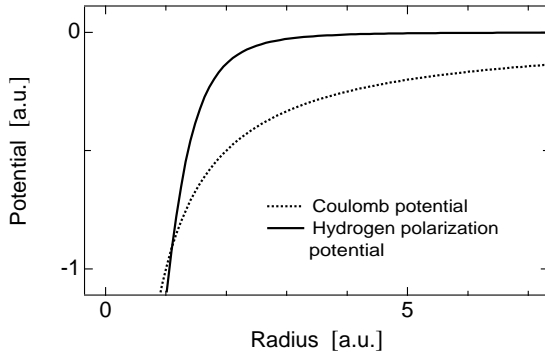
Figure 2.2.: Asymptotic potentials of H and H - : The asymptotic Coulomb potential, V(r) = -1/(r + r_0) r_0 = 18 \times 10^{-6} (proton radius), is compared to the polarisation potential (2.27) of H, V_{pol}(r) = -4.5/2(r^4 + 1) , with no linear Stark effect.
