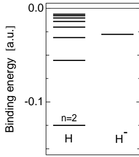
Figure 2.1.: Binding energies of H and H - : Energy levels for H and H - with respect to their ionisation/detachment limits. The ground state binding energies of H, 0.5 a.u., and H - , approx. 0.025 a.u., differ by roughly one order of magnitude, reflecting the different strength of the binding potential (see figure 2.2). Note also the absence of a Rydberg series for H - stemming from the lack of a long range asymptotic potential.
