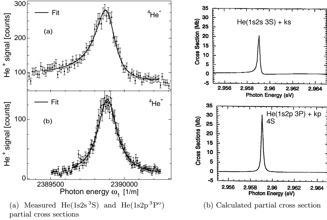
Figure 6.5.: Partial photodetachment cross section near the He - (1s3s4s 4 S) state: In the upper graph of part (a) we show a measurement of the He(1s2s 3 S)+e - (εs, εd) partial photodetachment cross sections of He - in the vicinity of the 1s3s4s 4 S resonance, and in the lower graph of part (a) a measurement of the He(1s2p 3 P o )+e - (εp) partial photodetachment cross sections of the same state. The use of co-propagating laser (ω 1 ) and ion beams causes the resonance to be Doppler shifted by 3 089 m -1 to the blue. The solid line is a fit to the data using equation (3.23). The error bars represent the shot noise. Each data point represents 200 laser pulses in the upper graph of part (a) and 100 laser pulses in the lower graph of part (a). For a comparison of width and position see figure 6.7,6.8 and table 6.3. The partial cross sections in part (b) are calculated by Xi [130].
