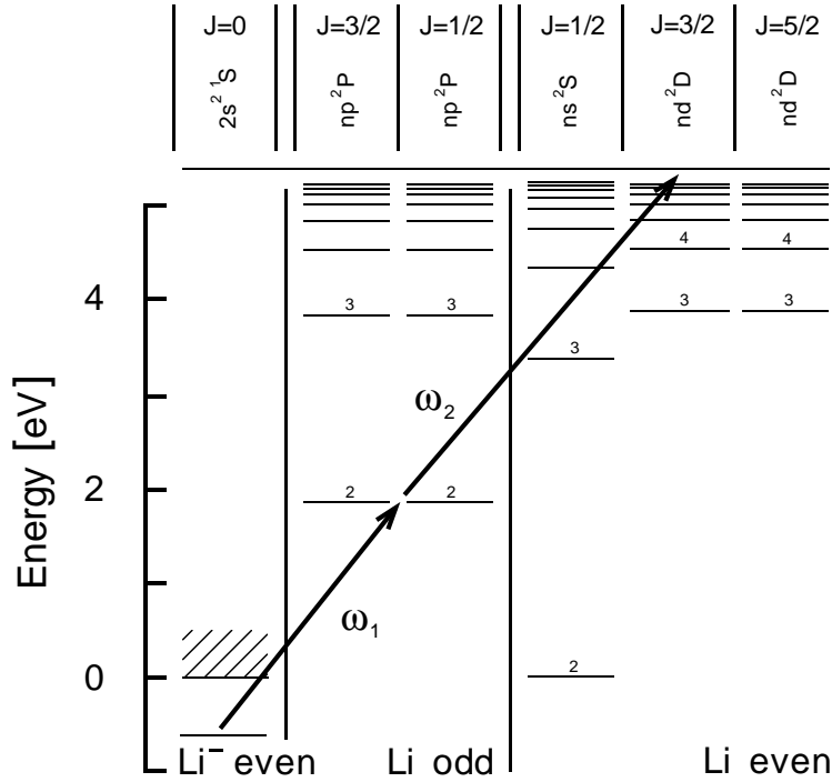
Figure 5.5.: Li^- excitation scheme I: Selected bound states of Li/Li^- grouped according to their parity and total angular momentum. The arrows indicate transitions induced in this experiment.
