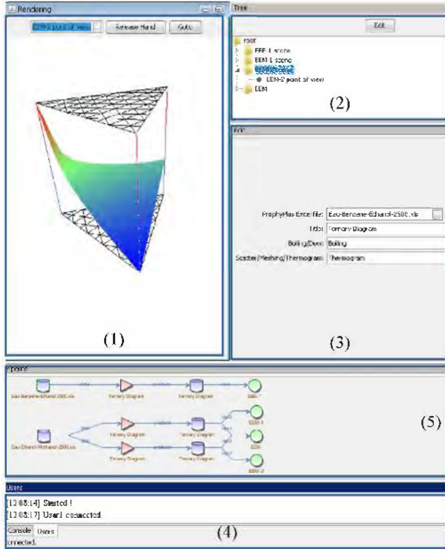
Fig. 5. Client interface.
