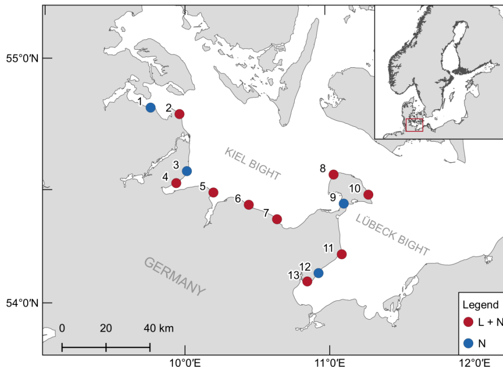
Figure 1. Geographical position of the 13 monitoring stations. Colors indicate if only samples for dissolved inorganic nutrients were taken (N) or in addition a logger station was deployed (L+N).
